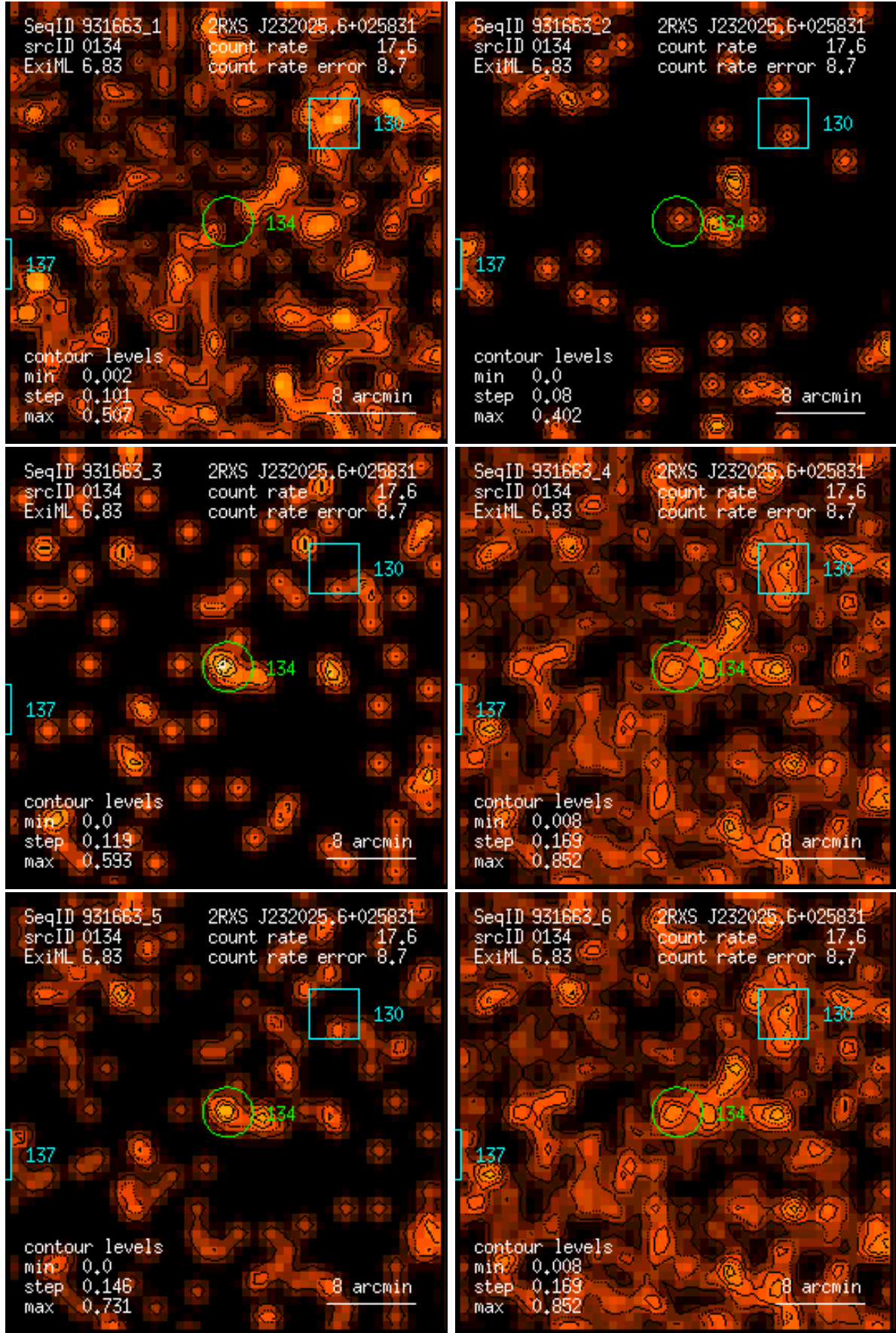
Figure 134: RASS 931663: detection 0134: band rate images, Gaussian filter: (1) PSPC channels 11 – 41, (2) 52 – 90, (3) 91 – 201, (4) 11 – 235, (5) 52 – 201, (6) 11 – 201. Broad band rates in counts/ks. Band rate contour levels in counts/ks/arcmin 2 .
