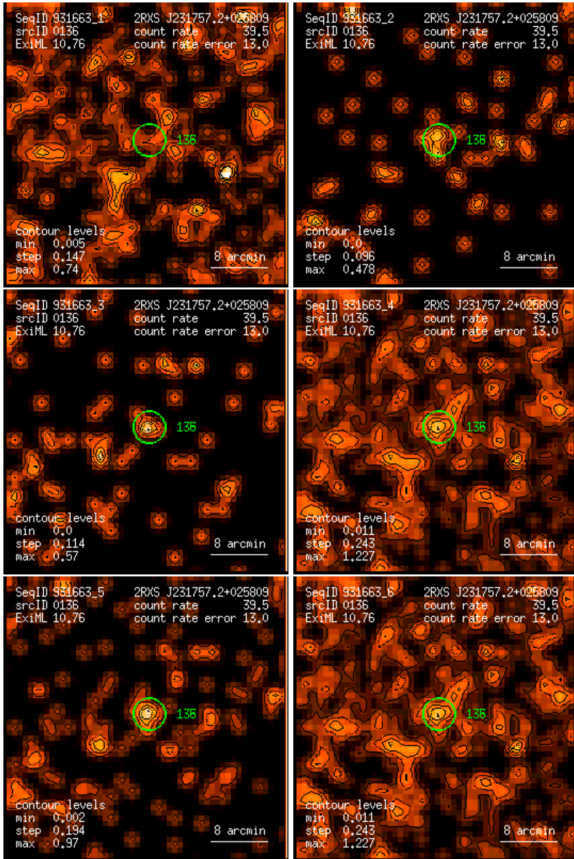
Figure 136: RASS 931663: detection 0136: band rate images, Gaussian filter: (1) PSPC channels 11 – 41, (2) 52 – 90, (3) 91 – 201, (4) 11 – 235, (5) 52 – 201, (6) 11 – 201. Broad band rates in counts/ks. Band rate contour levels in counts/ks/arcmin 2 .
