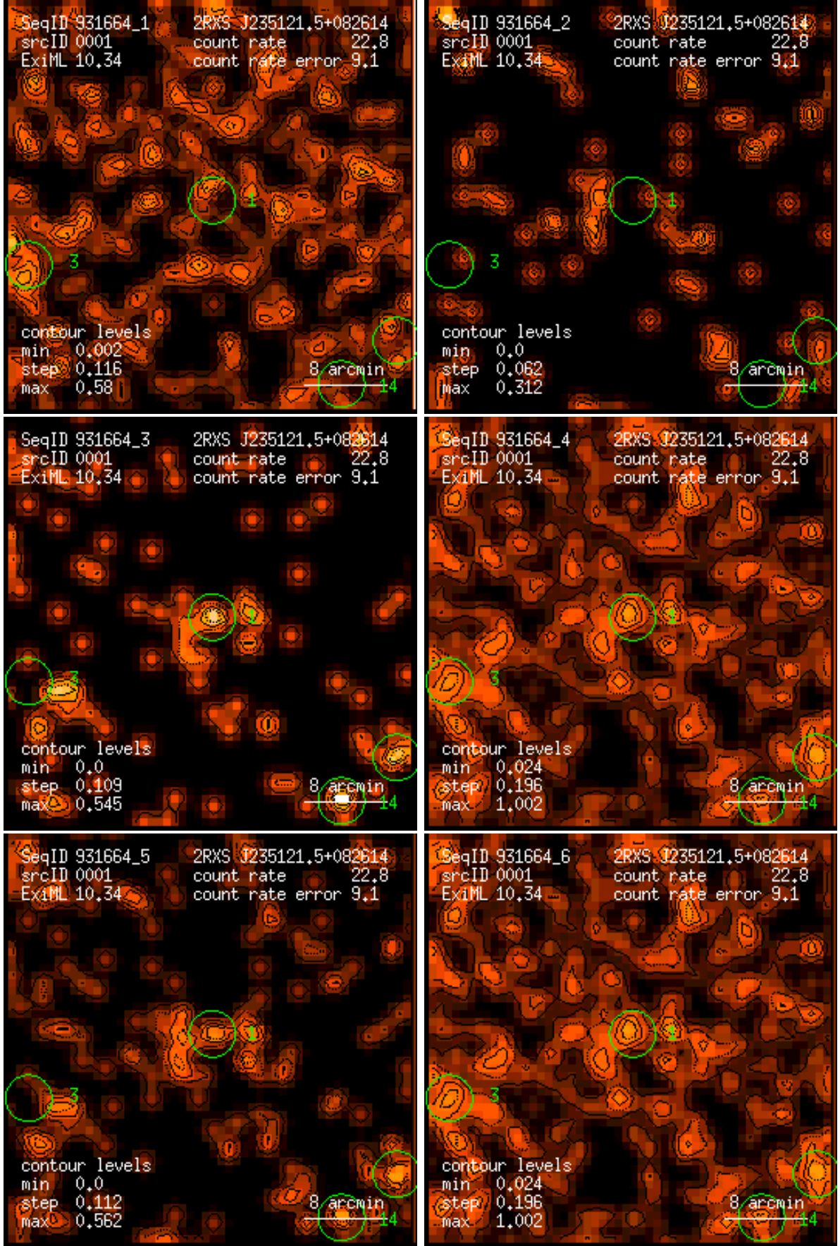
Figure 1: RASS 931664: detection 0001: band rate images, Gaussian filter: (1) PSPC channels 11 – 41, (2) 52 – 90, (3) 91 – 201, (4) 11 – 235, (5) 52 – 201, (6) 11 – 201. Broad band rates in counts/ks. Band rate contour levels in counts/ks/arcmin 2 .
