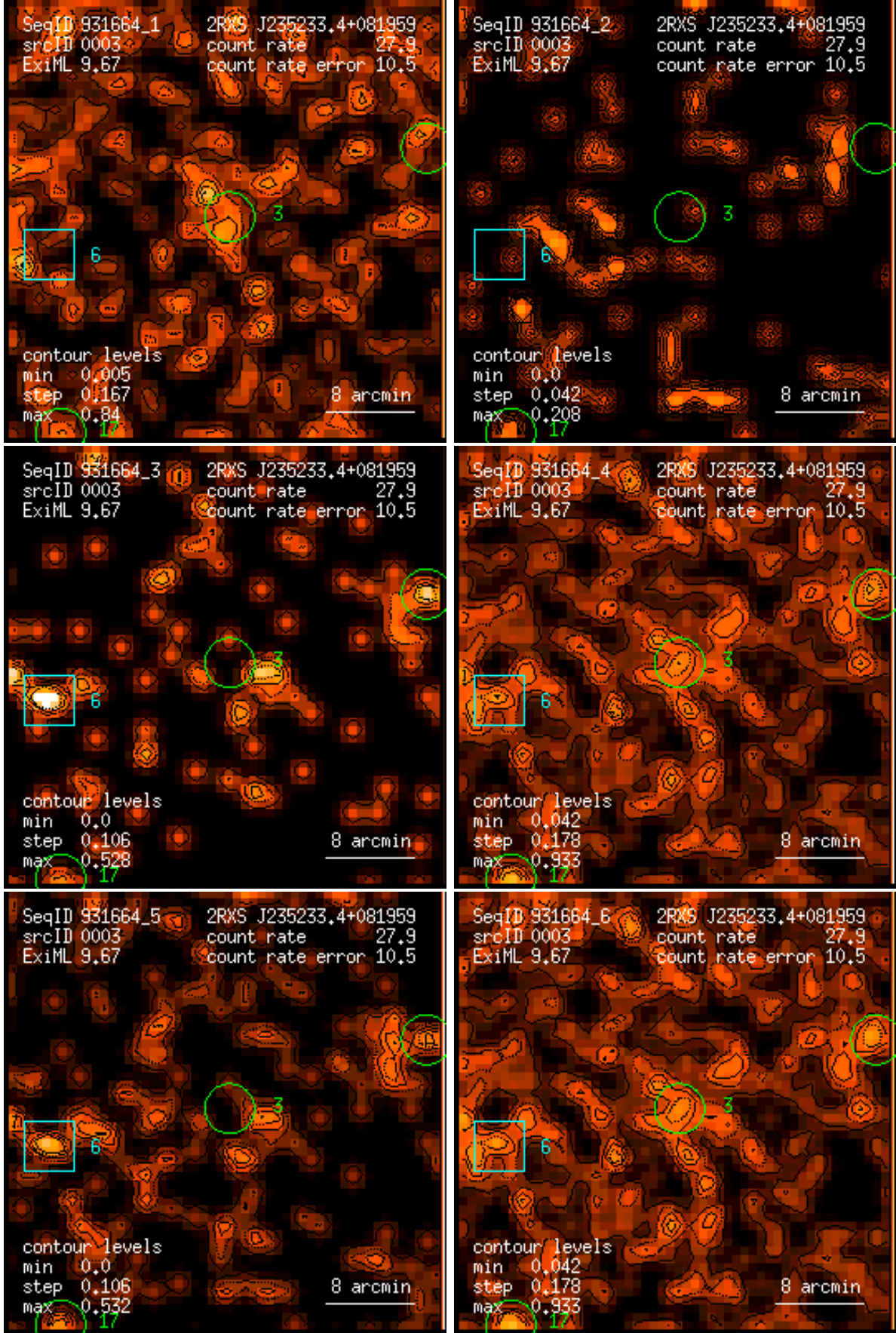
Figure 3: RASS 931664: detection 0003: band rate images, Gaussian filter: (1) PSPC channels 11 – 41, (2) 52 – 90, (3) 91 – 201, (4) 11 – 235, (5) 52 – 201, (6) 11 – 201. Broad band rates in counts/ks. Band rate contour levels in counts/ks/arcmin 2 .
