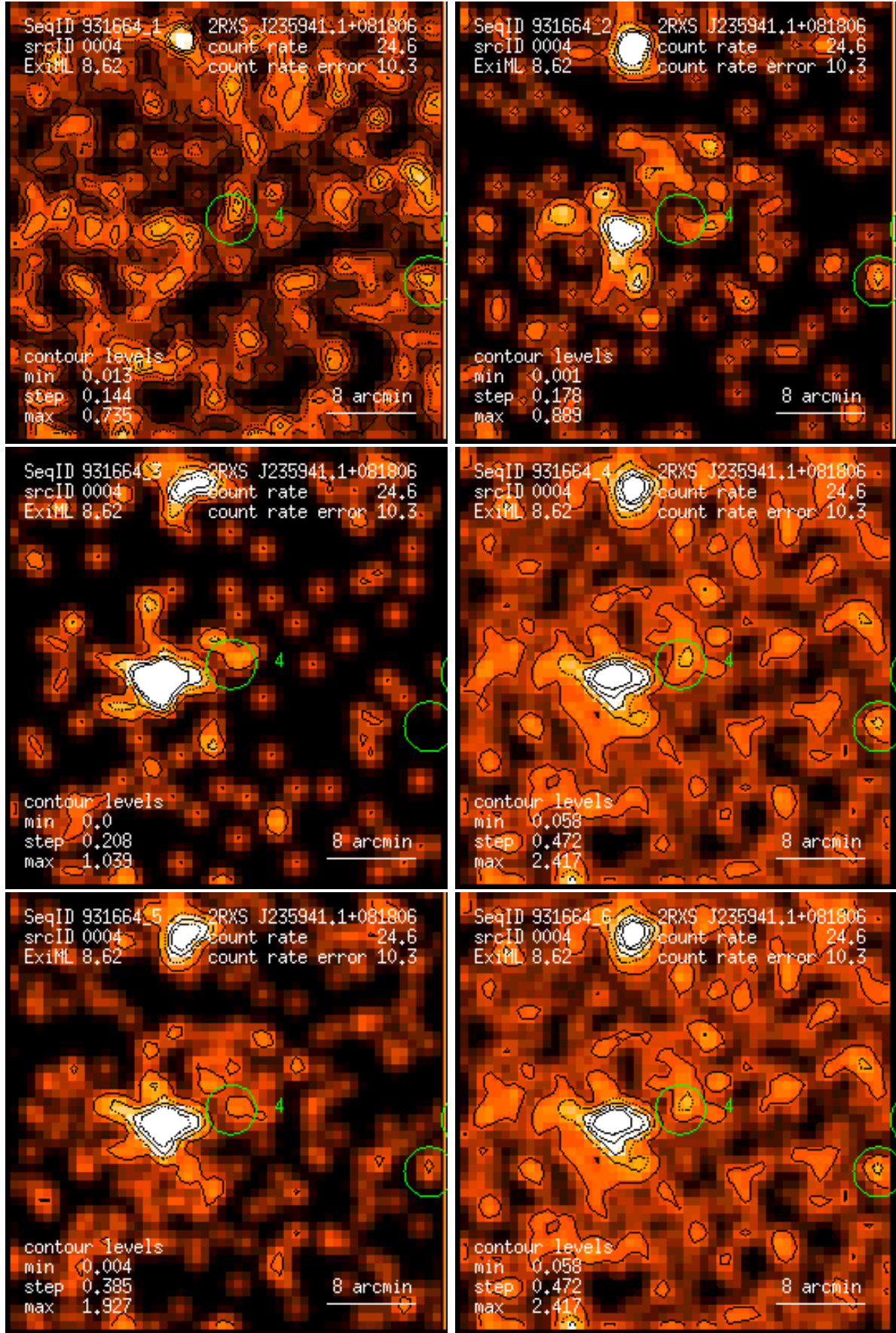
Figure 4: RASS 931664: detection 0004: band rate images, Gaussian filter: (1) PSPC channels 11 – 41, (2) 52 – 90, (3) 91 – 201, (4) 11 – 235, (5) 52 – 201, (6) 11 – 201. Broad band rates in counts/ks. Band rate contour levels in counts/ks/arcmin 2 .
