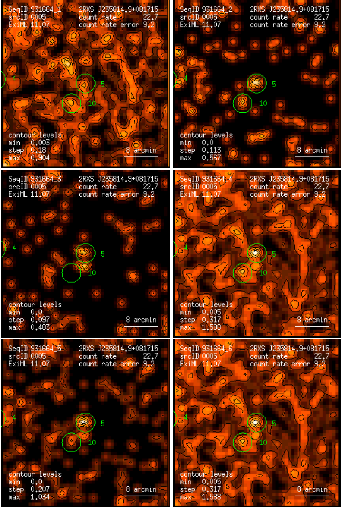
Figure 5: RASS 931664: detection 0005: band rate images, Gaussian filter: (1) PSPC channels 11 – 41, (2) 52 – 90, (3) 91 – 201, (4) 11 – 235, (5) 52 – 201, (6) 11 – 201. Broad band rates in counts/ks. Band rate contour levels in counts/ks/arcmin 2 .
