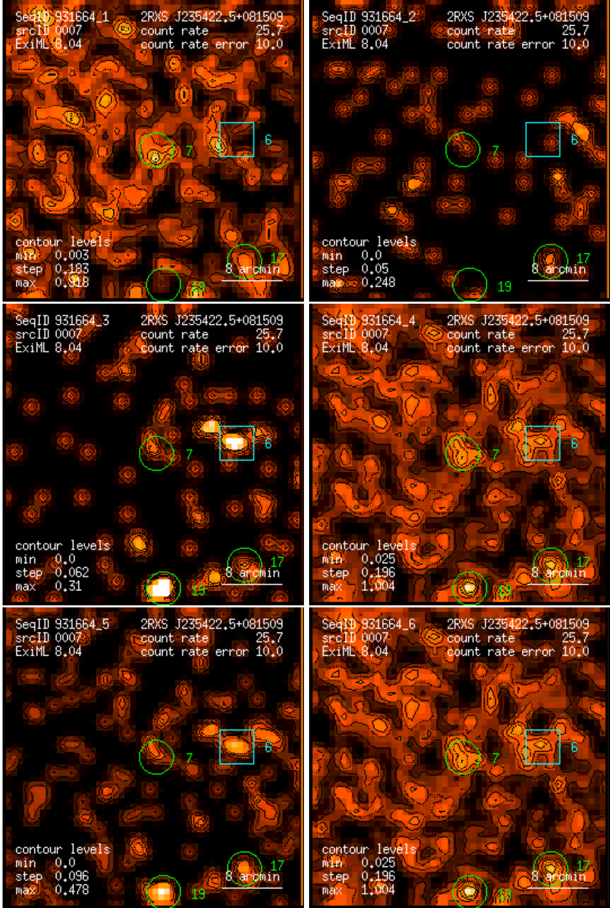
Figure 7: RASS 931664: detection 0007: band rate images, Gaussian filter: (1) PSPC channels 11 – 41, (2) 52 – 90, (3) 91 – 201, (4) 11 – 235, (5) 52 – 201, (6) 11 – 201. Broad band rates in counts/ks. Band rate contour levels in counts/ks/arcmin 2 .
