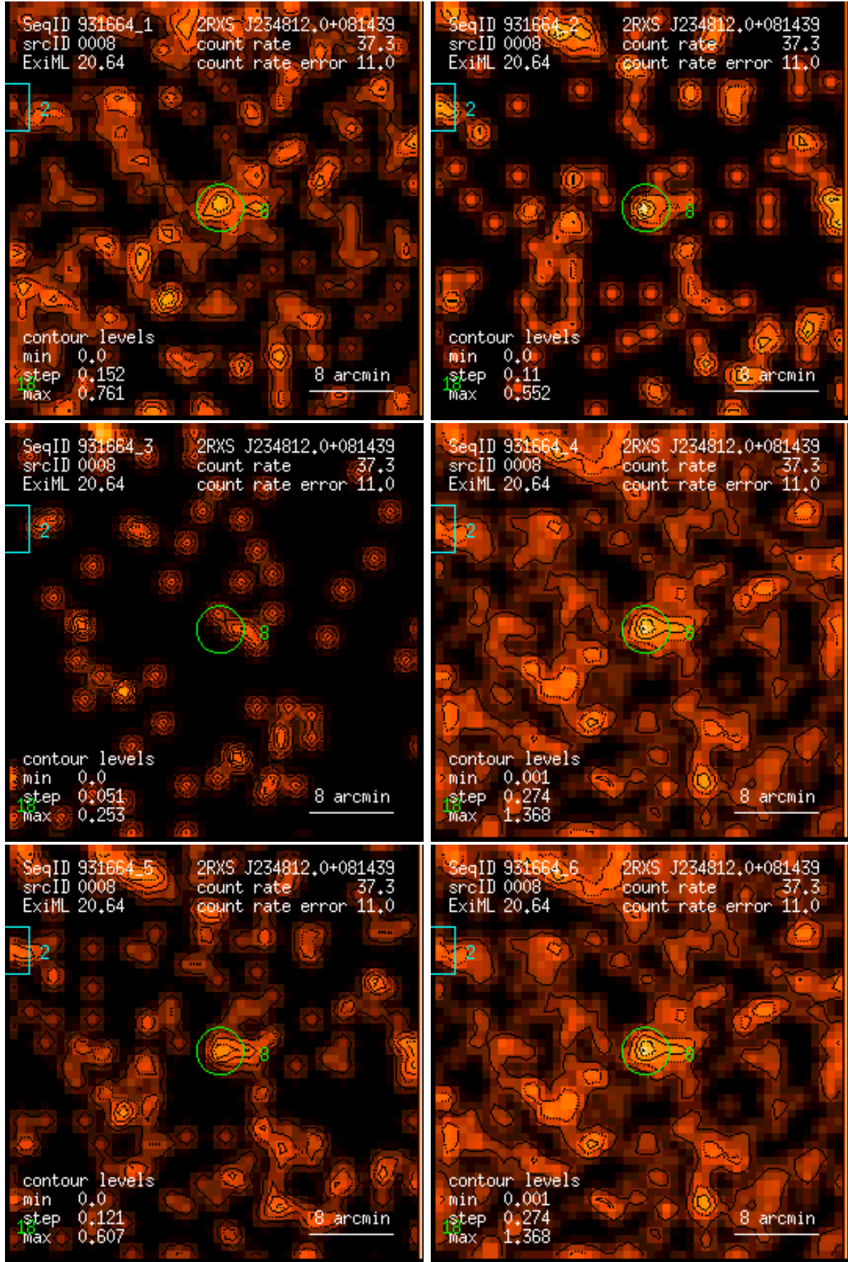
Figure 8: RASS 931664: detection 0008: band rate images, Gaussian filter: (1) PSPC channels 11 – 41, (2) 52 – 90, (3) 91 – 201, (4) 11 – 235, (5) 52 – 201, (6) 11 – 201. Broad band rates in counts/ks. Band rate contour levels in counts/ks/arcmin 2 .
