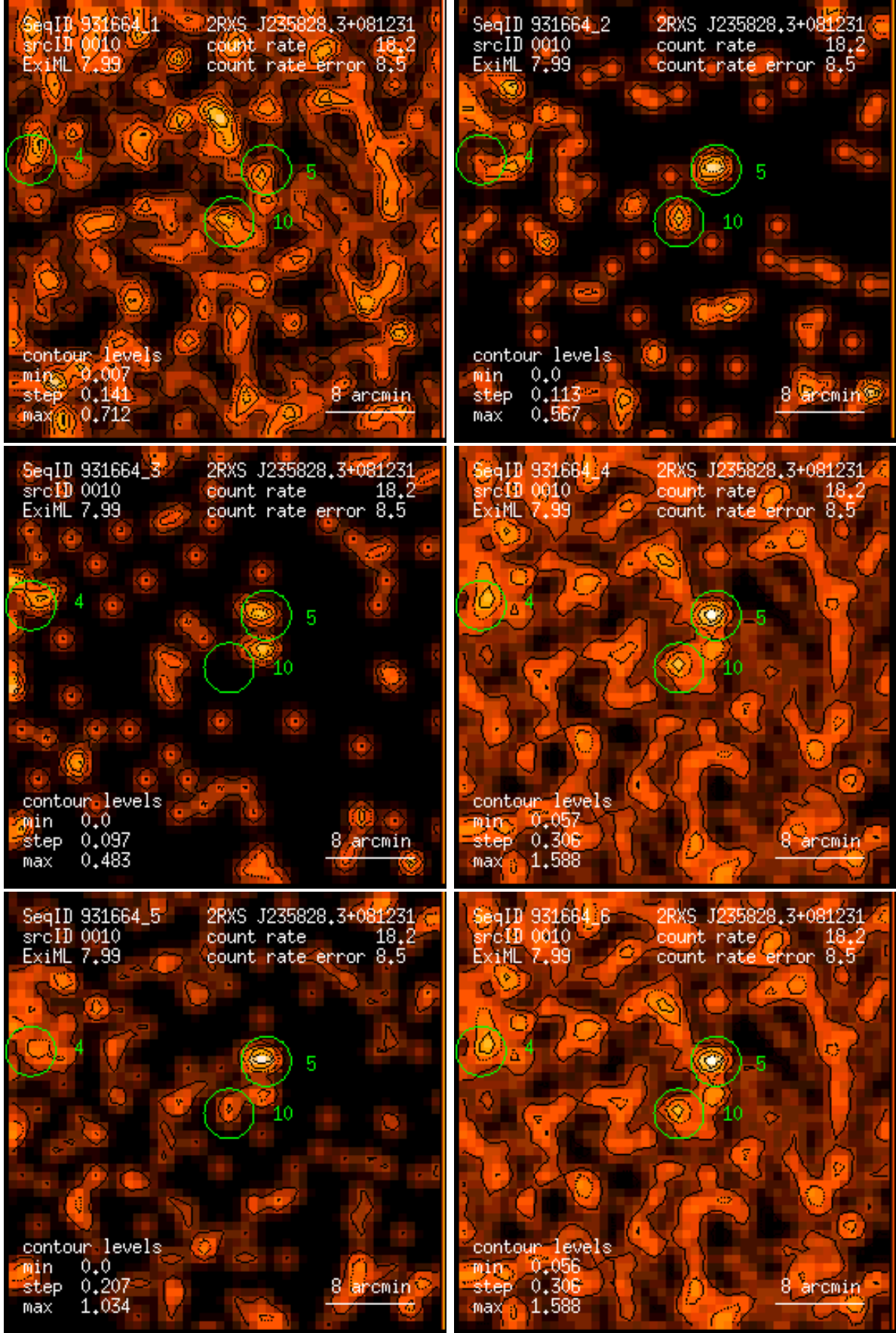
Figure 10: RASS 931664: detection 0010: band rate images, Gaussian filter: (1) PSPC channels 11 – 41, (2) 52 – 90, (3) 91 – 201, (4) 11 – 235, (5) 52 – 201, (6) 11 – 201. Broad band rates in counts/ks. Band rate contour levels in counts/ks/arcmin 2 .
