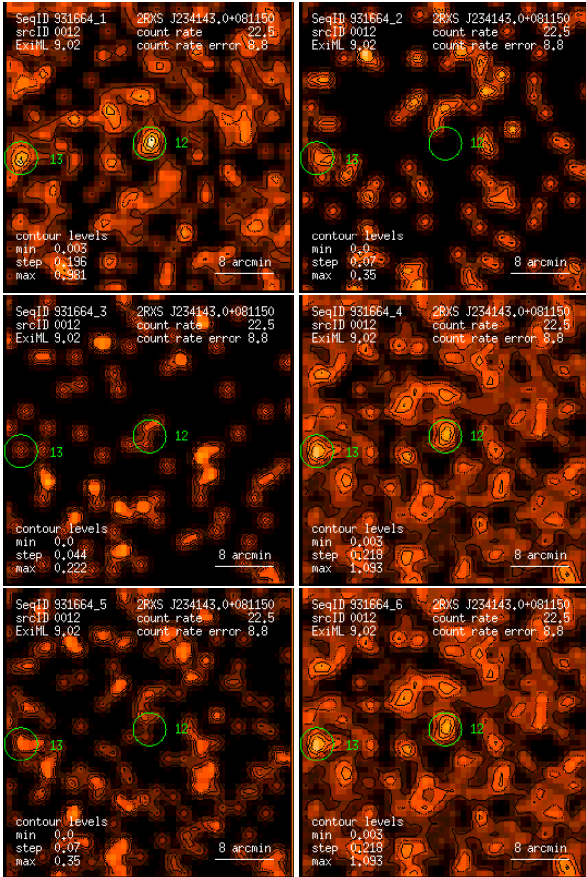
Figure 12: RASS 931664: detection 0012: band rate images, Gaussian filter: (1) PSPC channels 11 – 41, (2) 52 – 90, (3) 91 – 201, (4) 11 – 235, (5) 52 – 201, (6) 11 – 201. Broad band rates in counts/ks. Band rate contour levels in counts/ks/arcmin 2 .
