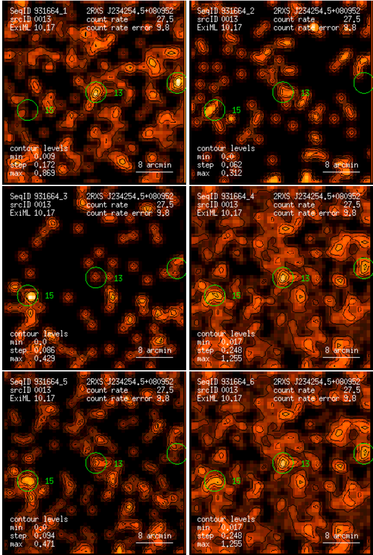
Figure 13: RASS 931664: detection 0013: band rate images, Gaussian filter: (1) PSPC channels 11 – 41, (2) 52 – 90, (3) 91 – 201, (4) 11 – 235, (5) 52 – 201, (6) 11 – 201. Broad band rates in counts/ks. Band rate contour levels in counts/ks/arcmin 2 .
