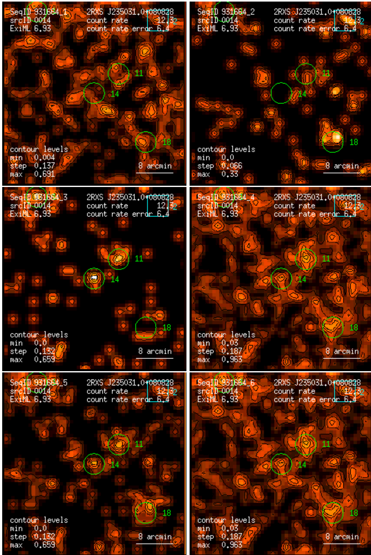
Figure 14: RASS 931664: detection 0014: band rate images, Gaussian filter: (1) PSPC channels 11 – 41, (2) 52 – 90, (3) 91 – 201, (4) 11 – 235, (5) 52 – 201, (6) 11 – 201. Broad band rates in counts/ks. Band rate contour levels in counts/ks/arcmin 2 .
