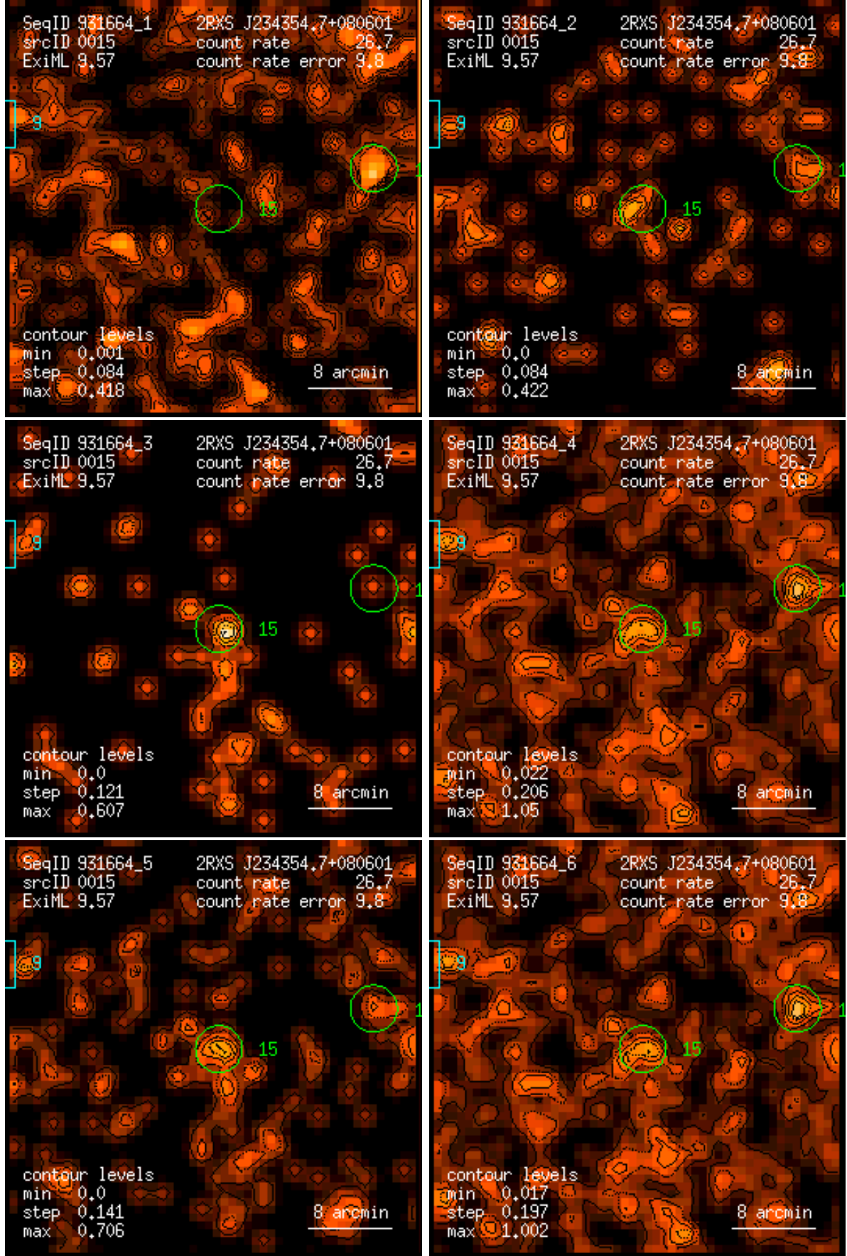
Figure 15: RASS 931664: detection 0015: band rate images, Gaussian filter: (1) PSPC channels 11 – 41, (2) 52 – 90, (3) 91 – 201, (4) 11 – 235, (5) 52 – 201, (6) 11 – 201. Broad band rates in counts/ks. Band rate contour levels in counts/ks/arcmin 2 .
