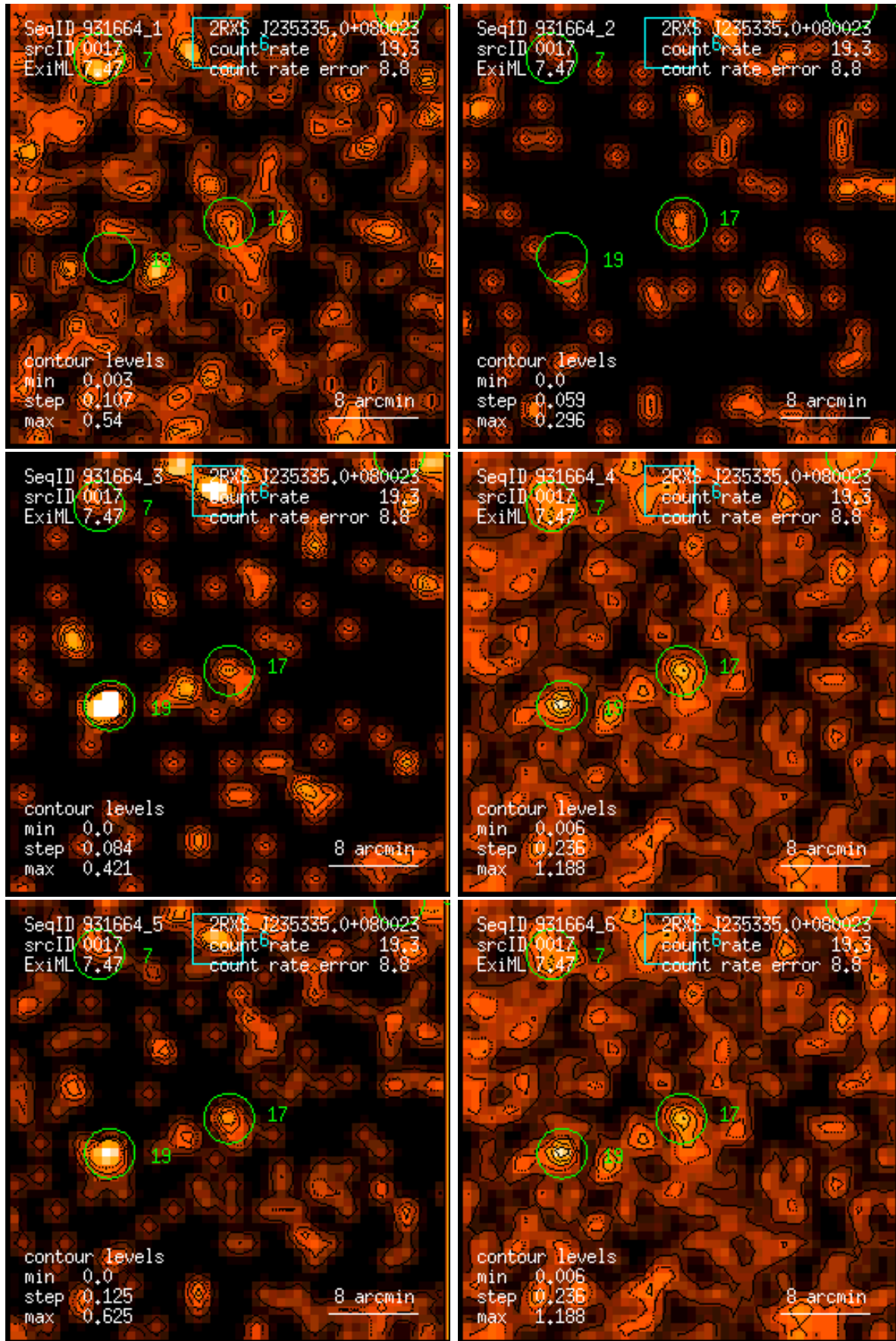
Figure 17: RASS 931664: detection 0017: band rate images, Gaussian filter: (1) PSPC channels 11 – 41, (2) 52 – 90, (3) 91 – 201, (4) 11 – 235, (5) 52 – 201, (6) 11 – 201. Broad band rates in counts/ks. Band rate contour levels in counts/ks/arcmin 2 .
