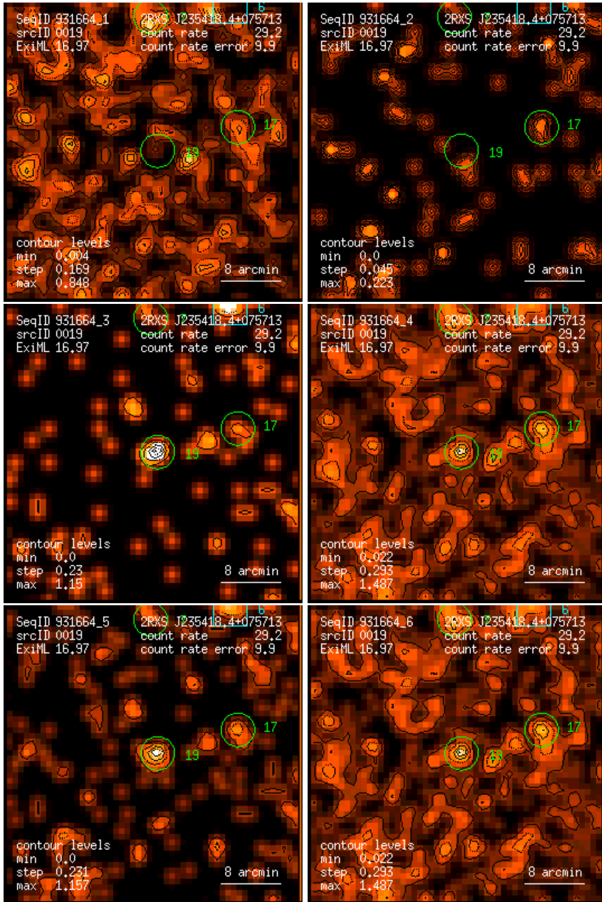
Figure 19: RASS 931664: detection 0019: band rate images, Gaussian filter: (1) PSPC channels 11 – 41, (2) 52 – 90, (3) 91 – 201, (4) 11 – 235, (5) 52 – 201, (6) 11 – 201. Broad band rates in counts/ks. Band rate contour levels in counts/ks/arcmin 2 .
