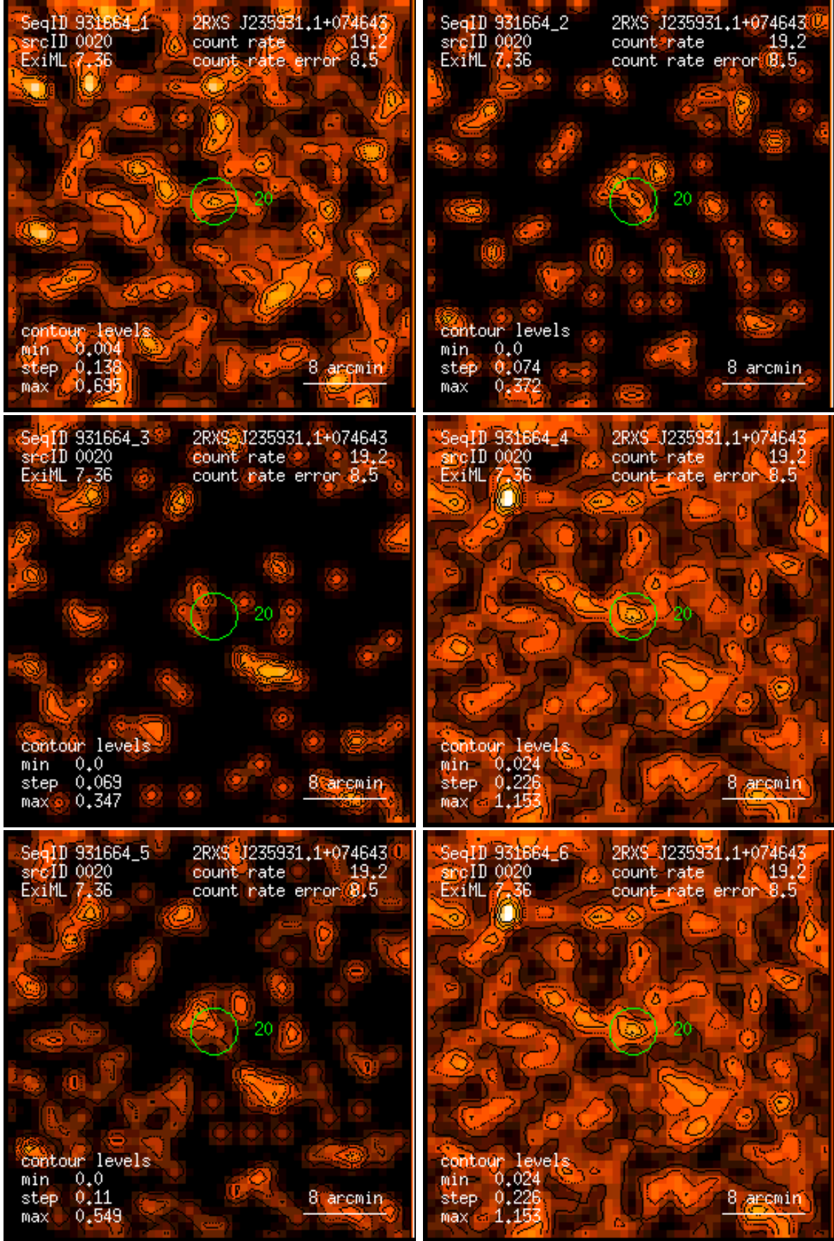
Figure 20: RASS 931664: detection 0020: band rate images, Gaussian filter: (1) PSPC channels 11 – 41, (2) 52 – 90, (3) 91 – 201, (4) 11 – 235, (5) 52 – 201, (6) 11 – 201. Broad band rates in counts/ks. Band rate contour levels in counts/ks/arcmin 2 .
