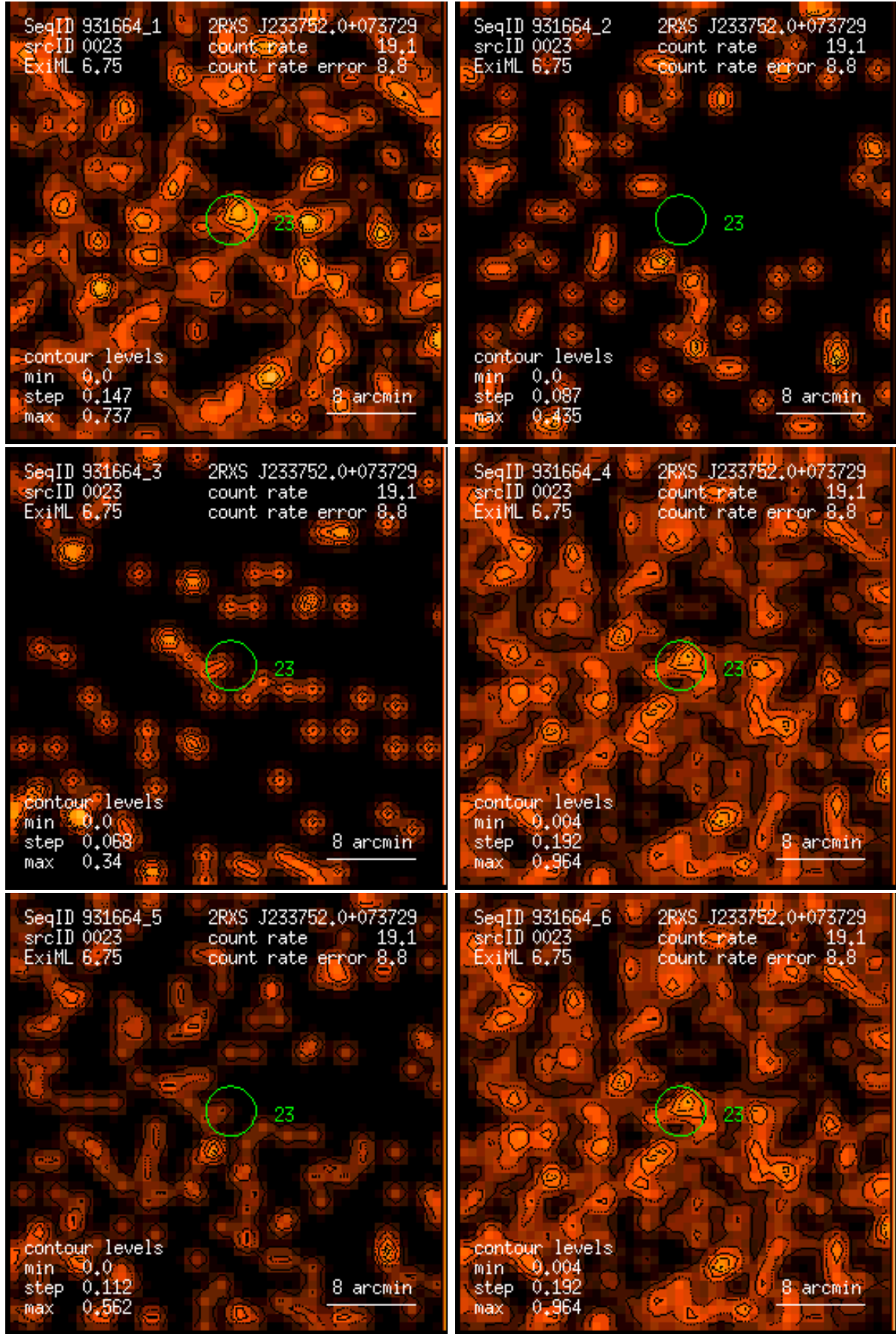
Figure 23: RASS 931664: detection 0023: band rate images, Gaussian filter: (1) PSPC channels 11 – 41, (2) 52 – 90, (3) 91 – 201, (4) 11 – 235, (5) 52 – 201, (6) 11 – 201. Broad band rates in counts/ks. Band rate contour levels in counts/ks/arcmin 2 .
