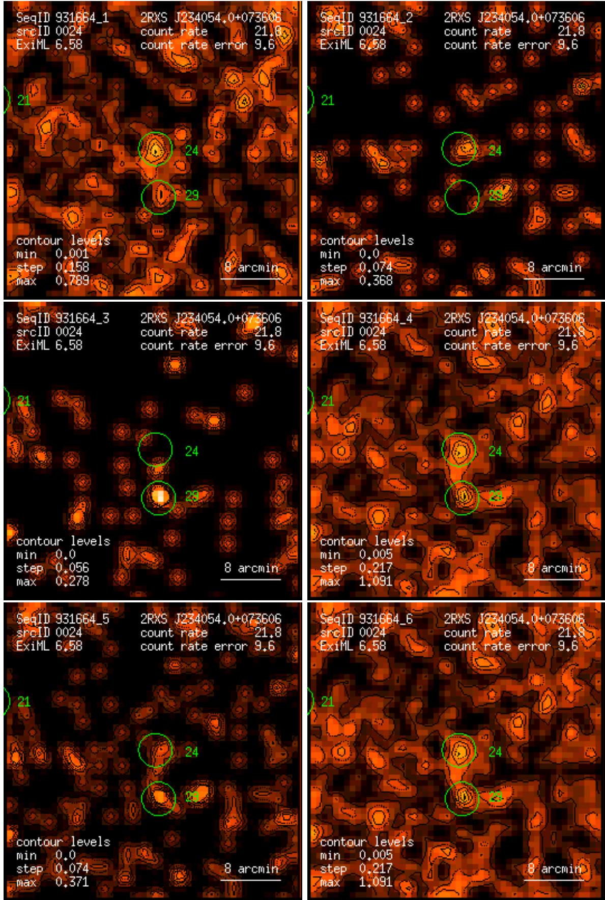
Figure 24: RASS 931664: detection 0024: band rate images, Gaussian filter: (1) PSPC channels 11 – 41, (2) 52 – 90, (3) 91 – 201, (4) 11 – 235, (5) 52 – 201, (6) 11 – 201. Broad band rates in counts/ks. Band rate contour levels in counts/ks/arcmin 2 .
