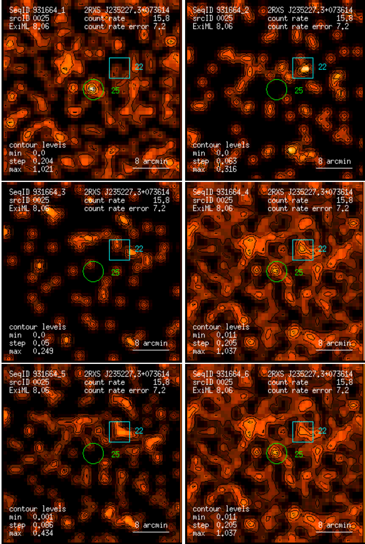
Figure 25: RASS 931664: detection 0025: band rate images, Gaussian filter: (1) PSPC channels 11 – 41, (2) 52 – 90, (3) 91 – 201, (4) 11 – 235, (5) 52 – 201, (6) 11 – 201. Broad band rates in counts/ks. Band rate contour levels in counts/ks/arcmin 2 .
