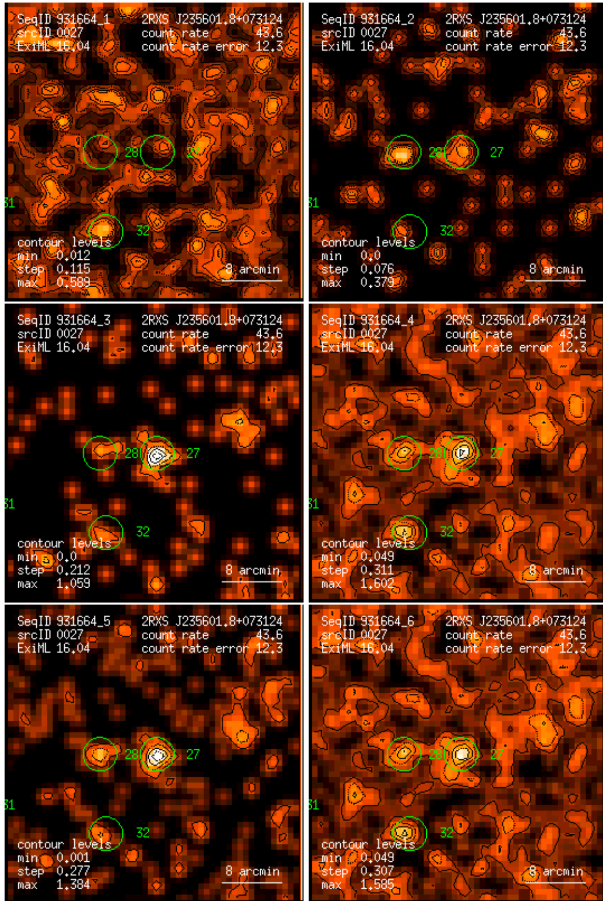
Figure 27: RASS 931664: detection 0027: band rate images, Gaussian filter: (1) PSPC channels 11 – 41, (2) 52 – 90, (3) 91 – 201, (4) 11 – 235, (5) 52 – 201, (6) 11 – 201. Broad band rates in counts/ks. Band rate contour levels in counts/ks/arcmin 2 .
