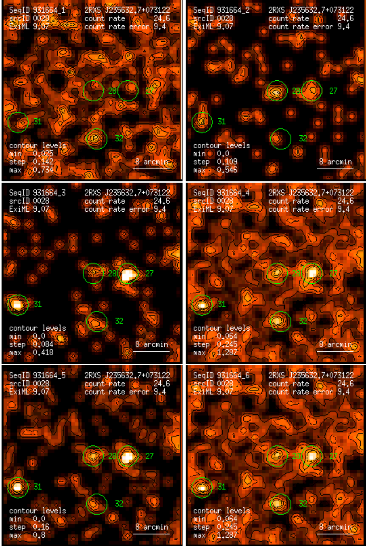
Figure 28: RASS 931664: detection 0028: band rate images, Gaussian filter: (1) PSPC channels 11 – 41, (2) 52 – 90, (3) 91 – 201, (4) 11 – 235, (5) 52 – 201, (6) 11 – 201. Broad band rates in counts/ks. Band rate contour levels in counts/ks/arcmin 2 .
