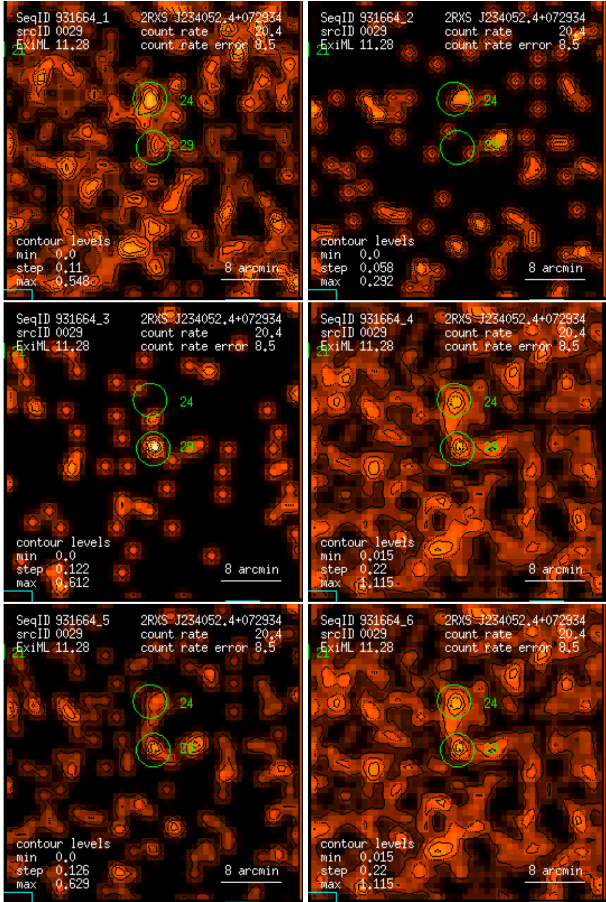
Figure 29: RASS 931664: detection 0029: band rate images, Gaussian filter: (1) PSPC channels 11 – 41, (2) 52 – 90, (3) 91 – 201, (4) 11 – 235, (5) 52 – 201, (6) 11 – 201. Broad band rates in counts/ks. Band rate contour levels in counts/ks/arcmin 2 .
