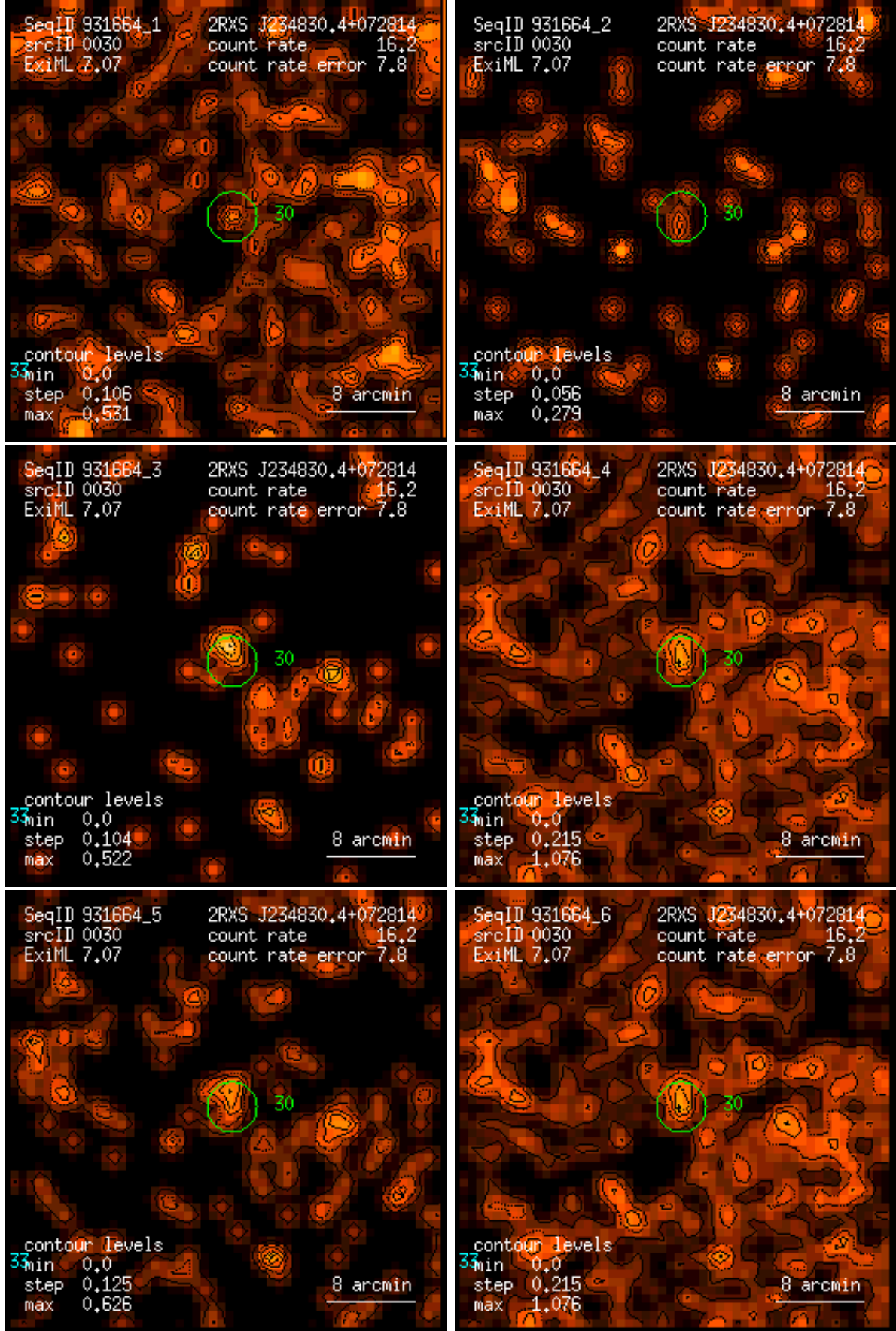
Figure 30: RASS 931664: detection 0030: band rate images, Gaussian filter: (1) PSPC channels 11 – 41, (2) 52 – 90, (3) 91 – 201, (4) 11 – 235, (5) 52 – 201, (6) 11 – 201. Broad band rates in counts/ks. Band rate contour levels in counts/ks/arcmin 2 .
