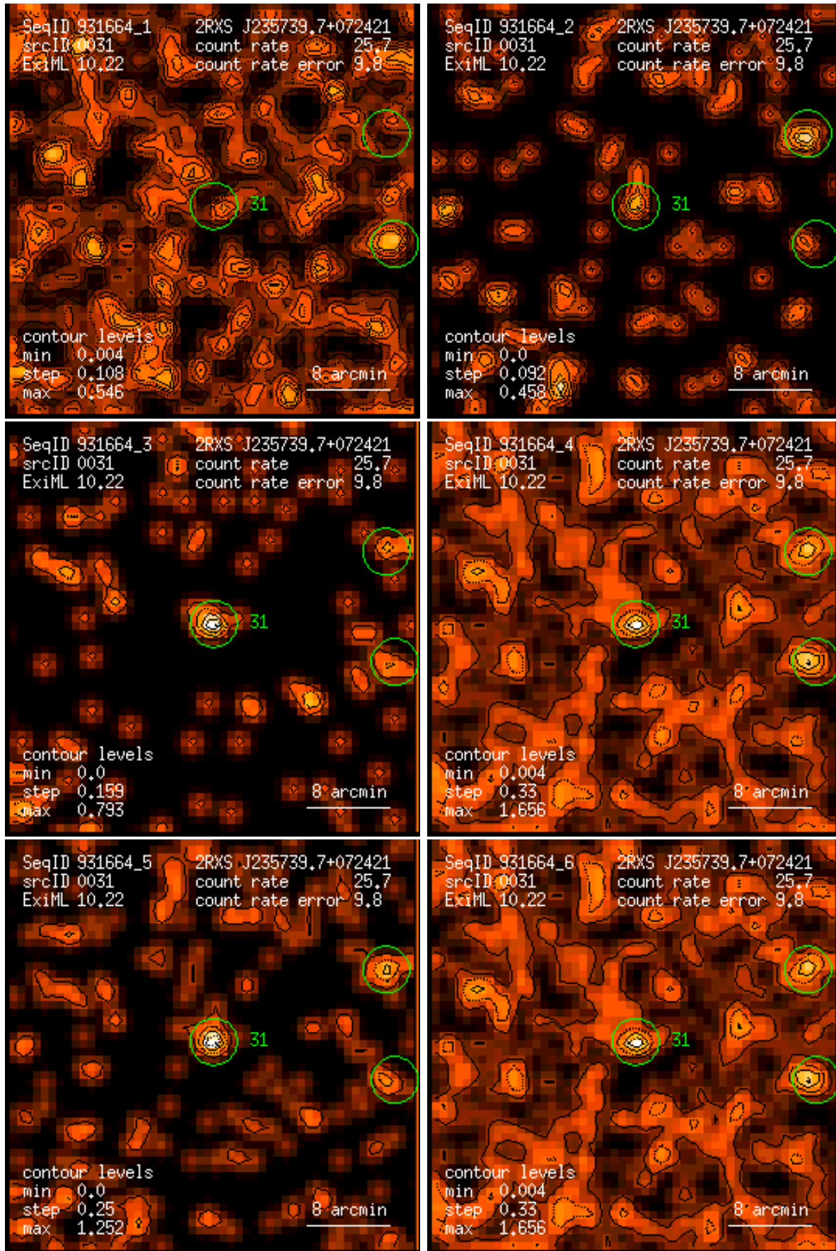
Figure 31: RASS 931664: detection 0031: band rate images, Gaussian filter: (1) PSPC channels 11 – 41, (2) 52 – 90, (3) 91 – 201, (4) 11 – 235, (5) 52 – 201, (6) 11 – 201. Broad band rates in counts/ks. Band rate contour levels in counts/ks/arcmin 2 .
