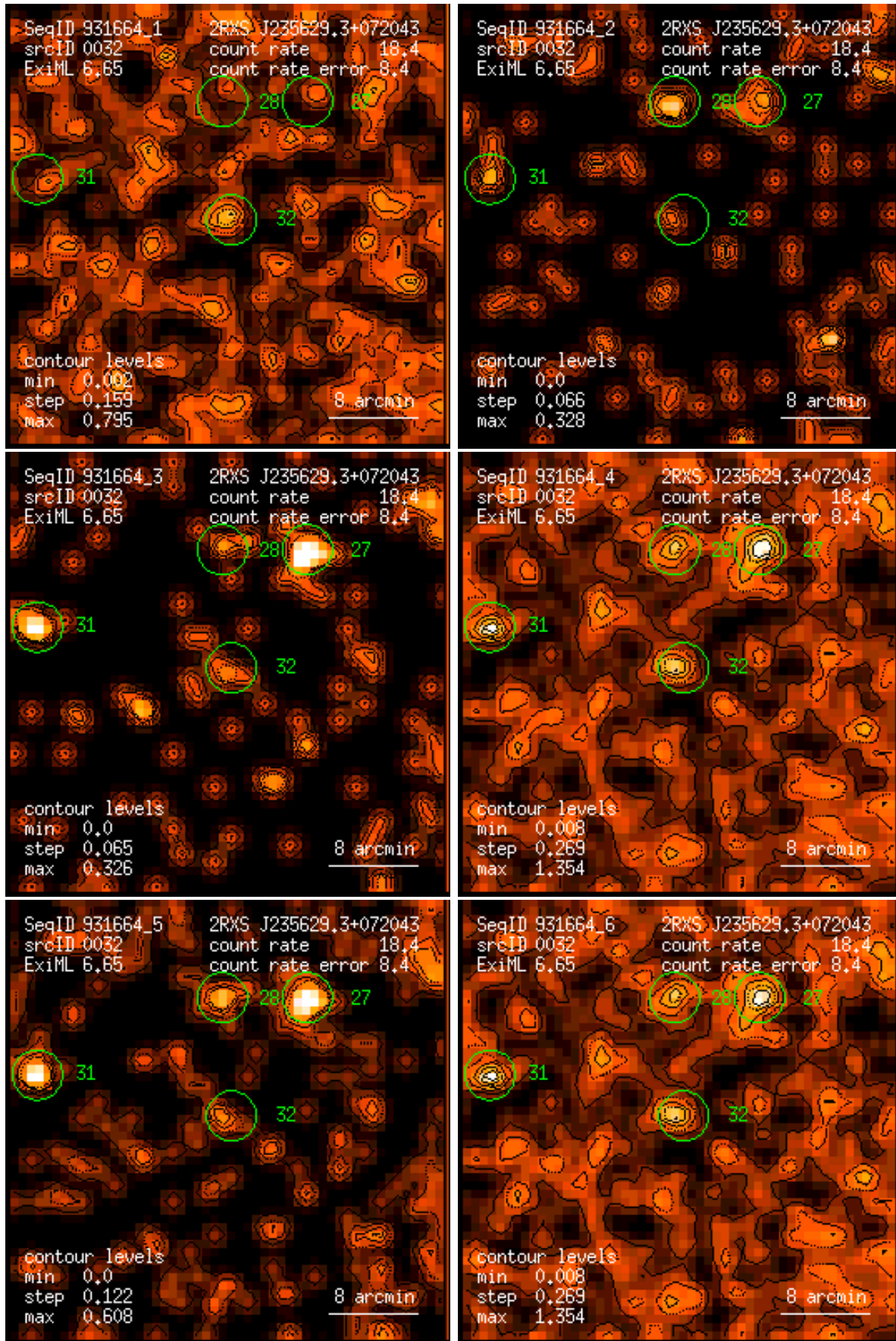
Figure 32: RASS 931664: detection 0032: band rate images, Gaussian filter: (1) PSPC channels 11 – 41, (2) 52 – 90, (3) 91 – 201, (4) 11 – 235, (5) 52 – 201, (6) 11 – 201. Broad band rates in counts/ks. Band rate contour levels in counts/ks/arcmin 2 .
