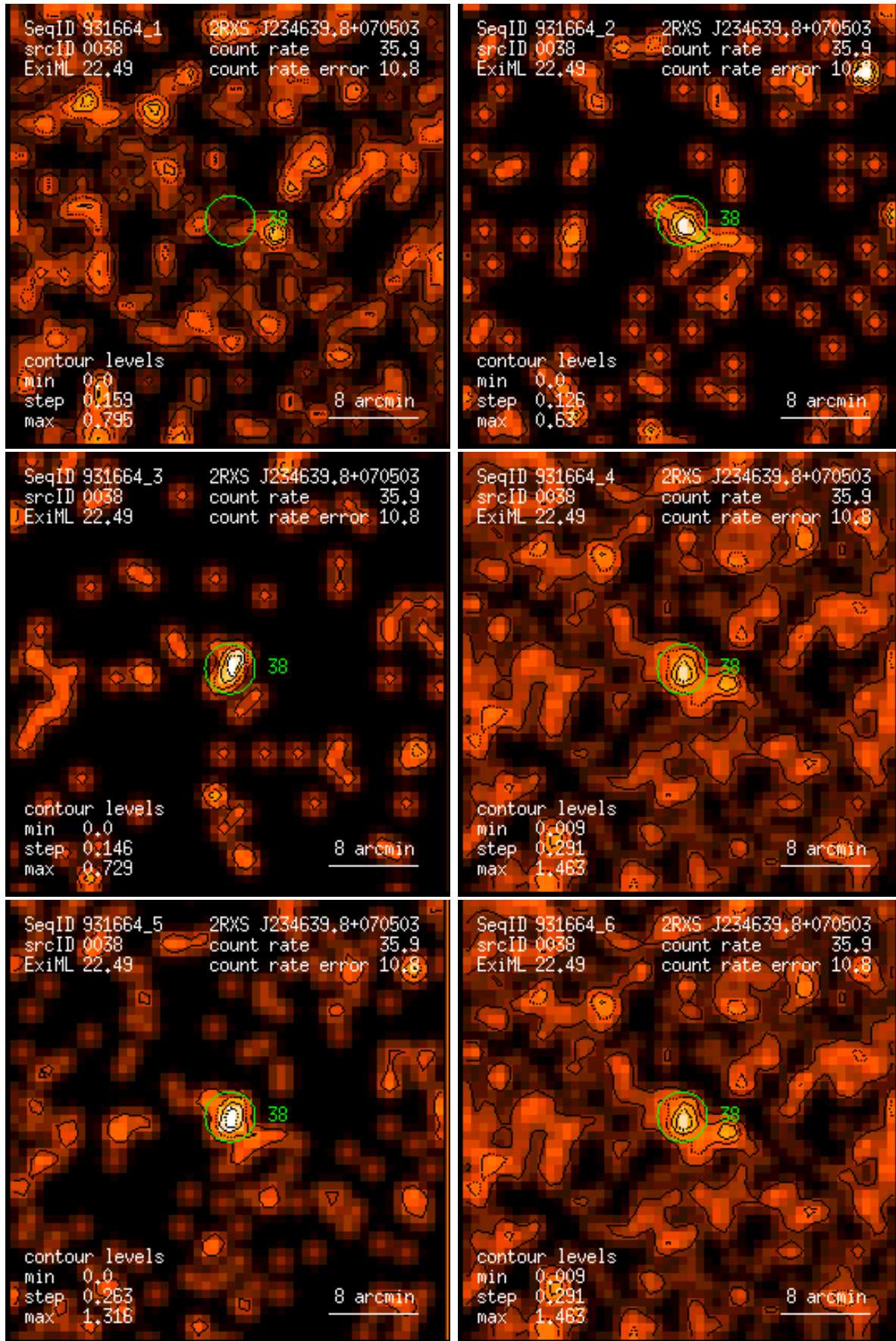
Figure 38: RASS 931664: detection 0038: band rate images, Gaussian filter: (1) PSPC channels 11 – 41, (2) 52 – 90, (3) 91 – 201, (4) 11 – 235, (5) 52 – 201, (6) 11 – 201. Broad band rates in counts/ks. Band rate contour levels in counts/ks/arcmin 2 .
