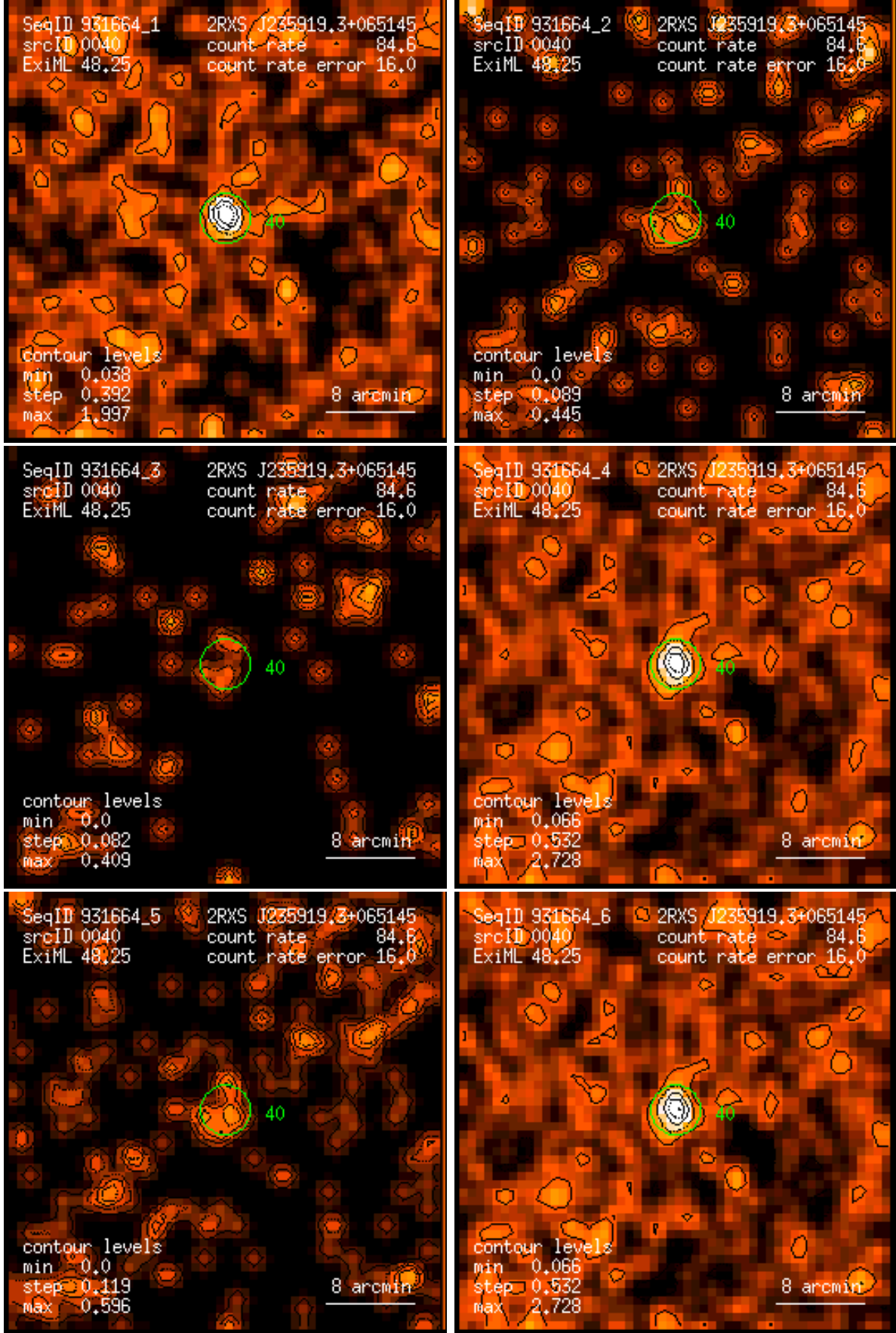
Figure 40: RASS 931664: detection 0040: band rate images, Gaussian filter: (1) PSPC channels 11 – 41, (2) 52 – 90, (3) 91 – 201, (4) 11 – 235, (5) 52 – 201, (6) 11 – 201. Broad band rates in counts/ks. Band rate contour levels in counts/ks/arcmin 2 .
