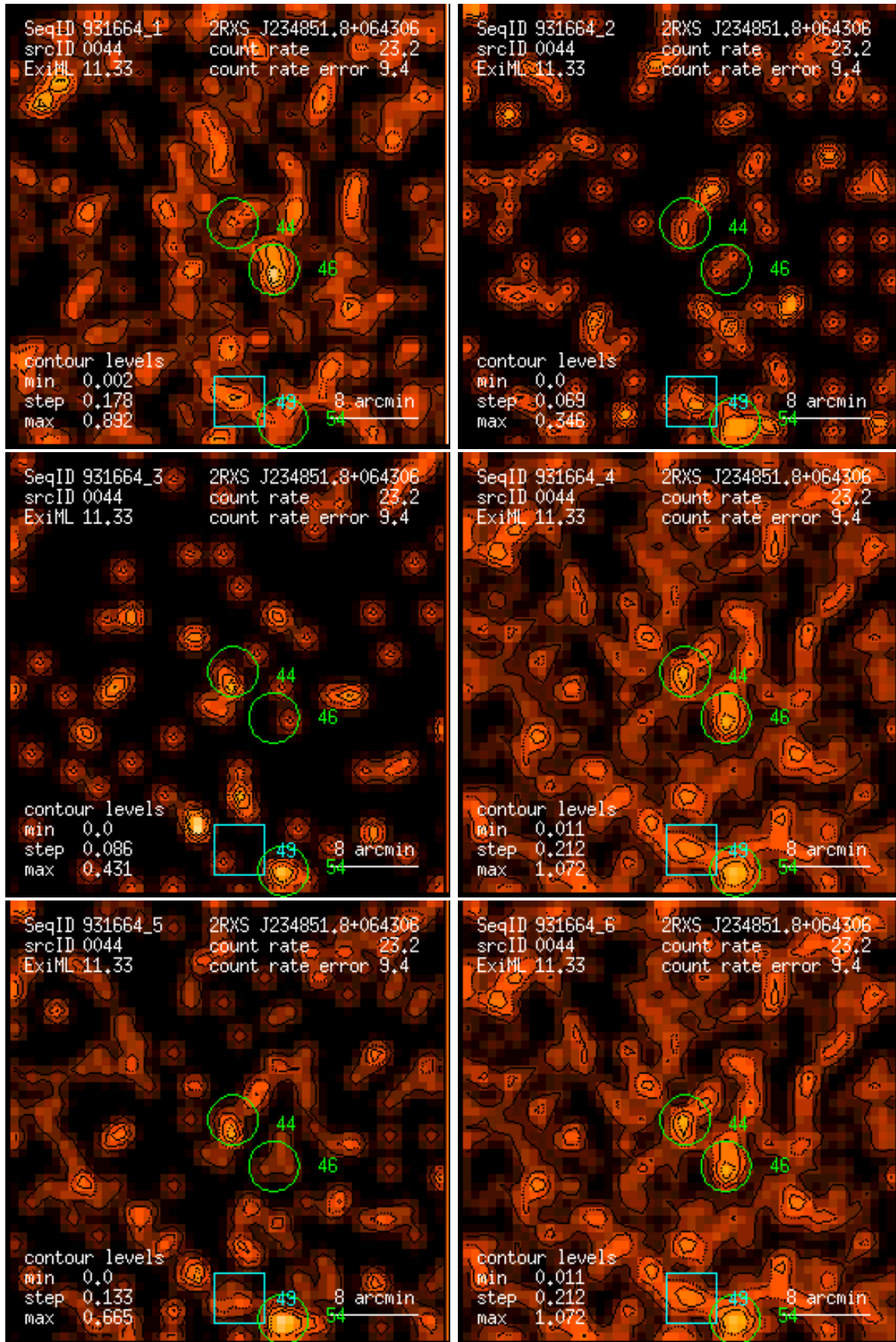
Figure 44: RASS 931664: detection 0044: band rate images, Gaussian filter: (1) PSPC channels 11 – 41, (2) 52 – 90, (3) 91 – 201, (4) 11 – 235, (5) 52 – 201, (6) 11 – 201. Broad band rates in counts/ks. Band rate contour levels in counts/ks/arcmin 2 .
