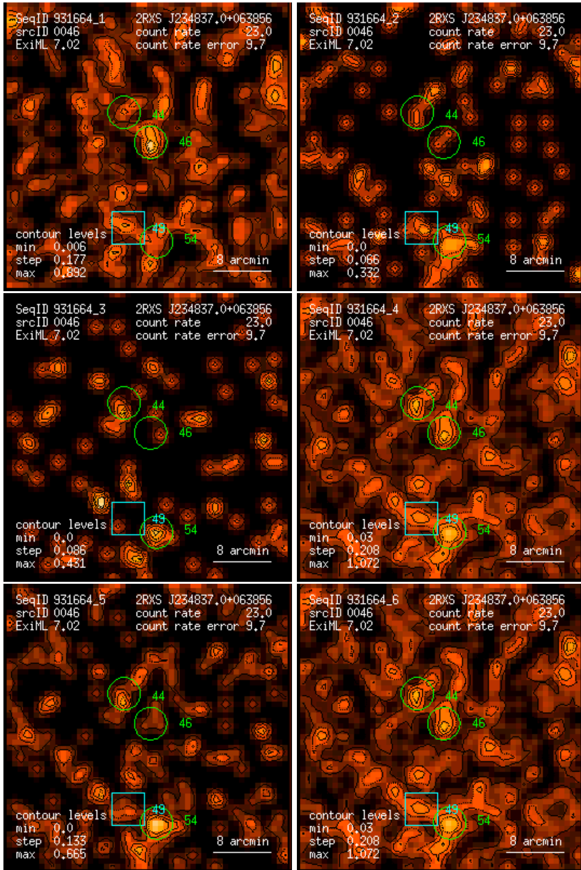
Figure 46: RASS 931664: detection 0046: band rate images, Gaussian filter: (1) PSPC channels 11 – 41, (2) 52 – 90, (3) 91 – 201, (4) 11 – 235, (5) 52 – 201, (6) 11 – 201. Broad band rates in counts/ks. Band rate contour levels in counts/ks/arcmin 2 .
