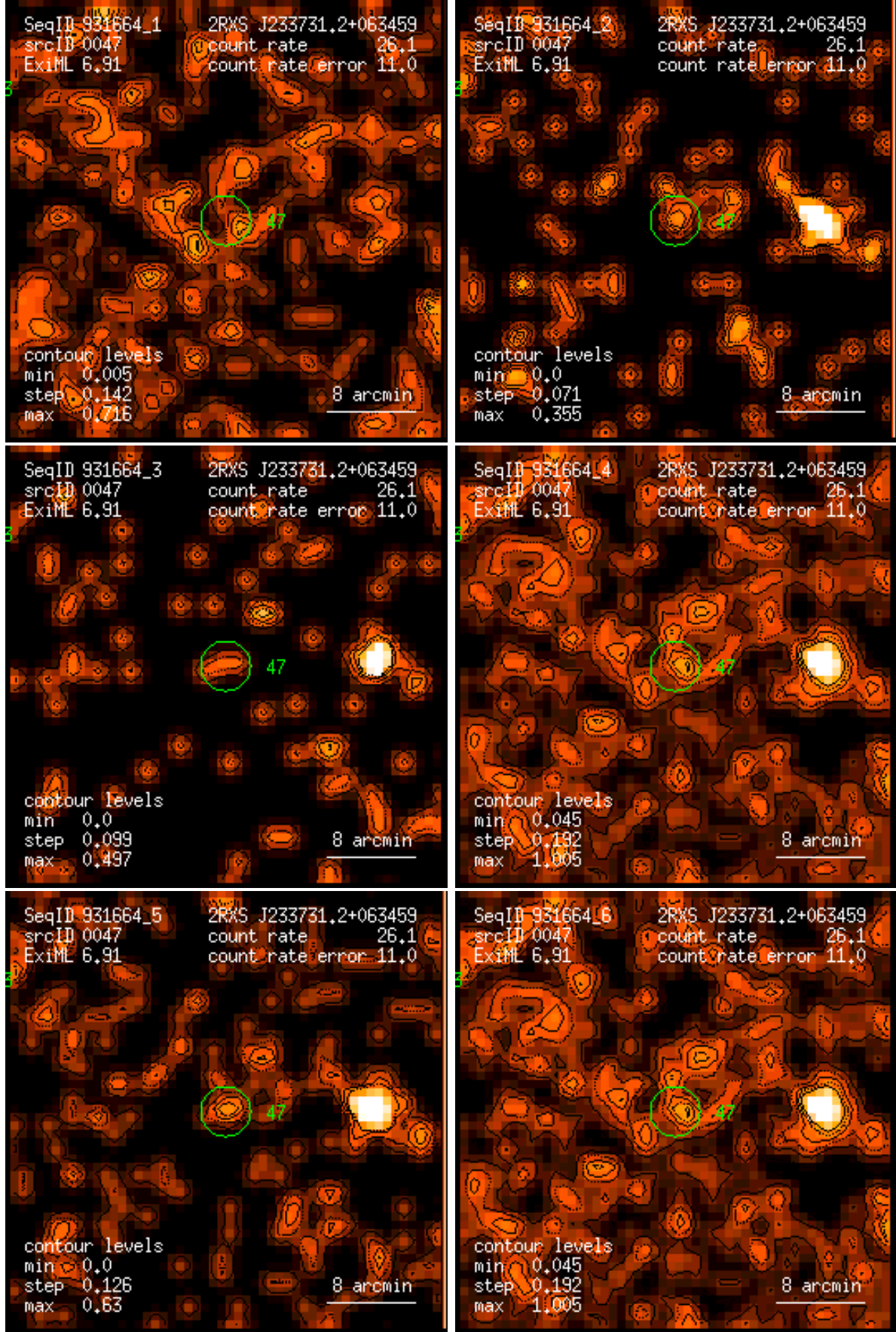
Figure 47: RASS 931664: detection 0047: band rate images, Gaussian filter: (1) PSPC channels 11 – 41, (2) 52 – 90, (3) 91 – 201, (4) 11 – 235, (5) 52 – 201, (6) 11 – 201. Broad band rates in counts/ks. Band rate contour levels in counts/ks/arcmin 2 .
