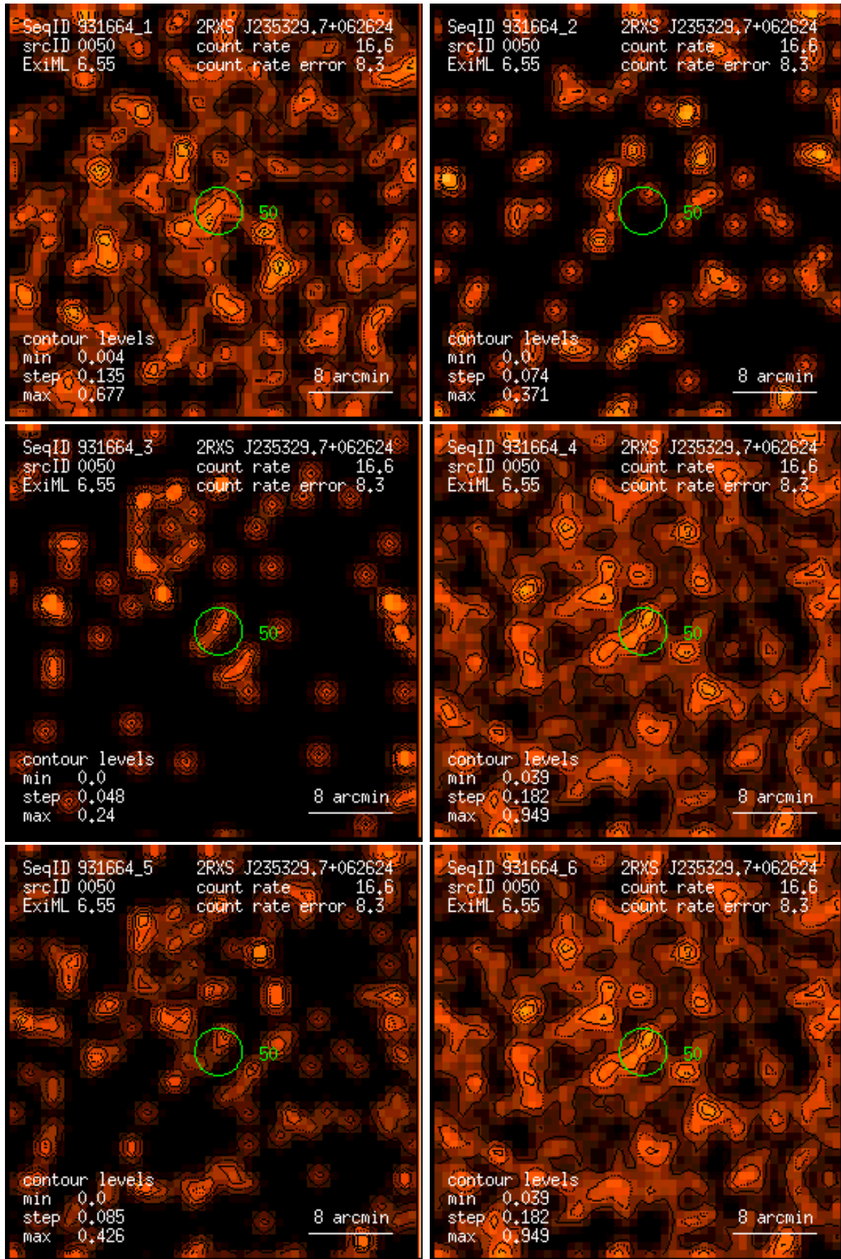
Figure 50: RASS 931664: detection 0050: band rate images, Gaussian filter: (1) PSPC channels 11 – 41, (2) 52 – 90, (3) 91 – 201, (4) 11 – 235, (5) 52 – 201, (6) 11 – 201. Broad band rates in counts/ks. Band rate contour levels in counts/ks/arcmin 2 .
