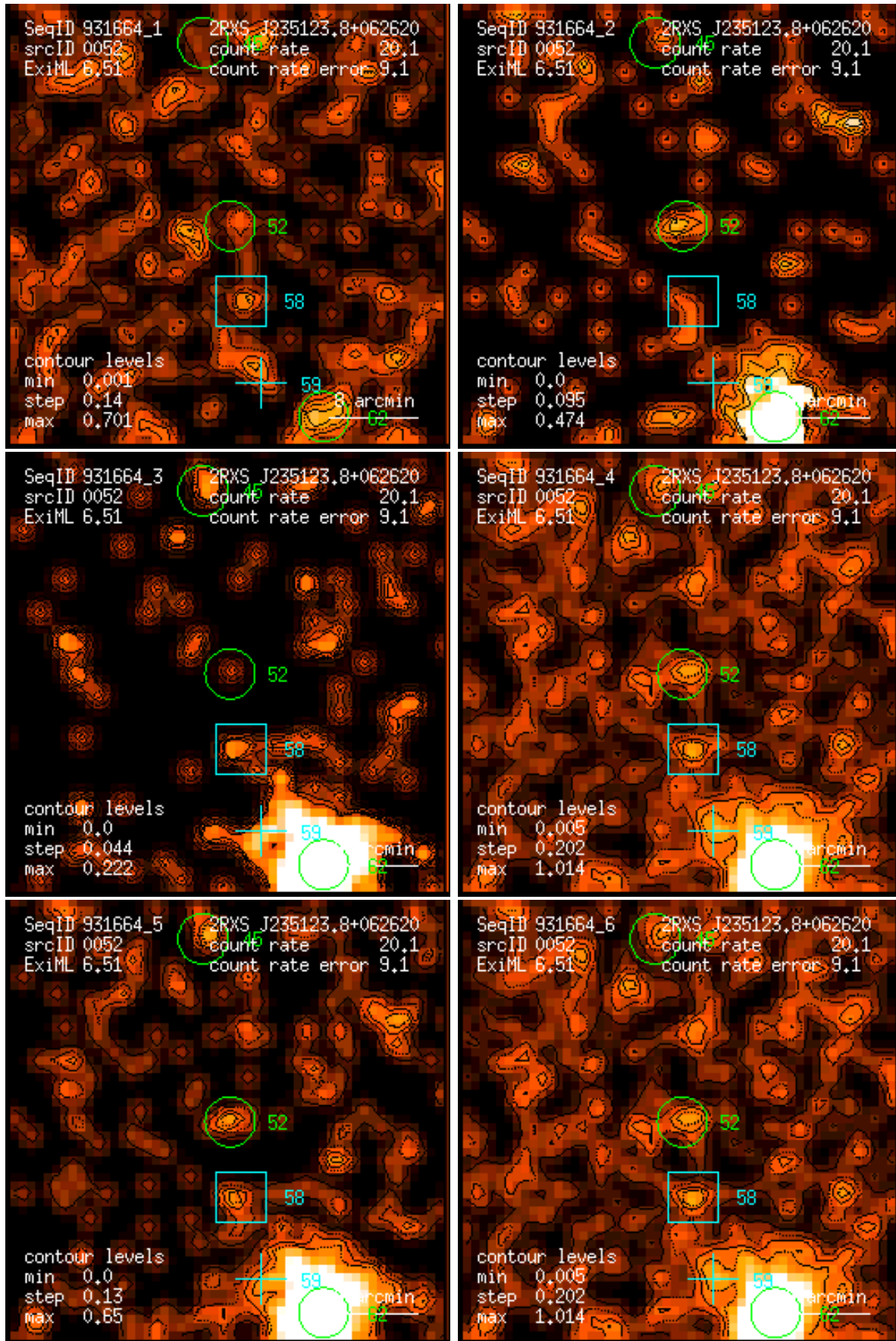
Figure 52: RASS 931664: detection 0052: band rate images, Gaussian filter: (1) PSPC channels 11 – 41, (2) 52 – 90, (3) 91 – 201, (4) 11 – 235, (5) 52 – 201, (6) 11 – 201. Broad band rates in counts/ks. Band rate contour levels in counts/ks/arcmin 2 .
