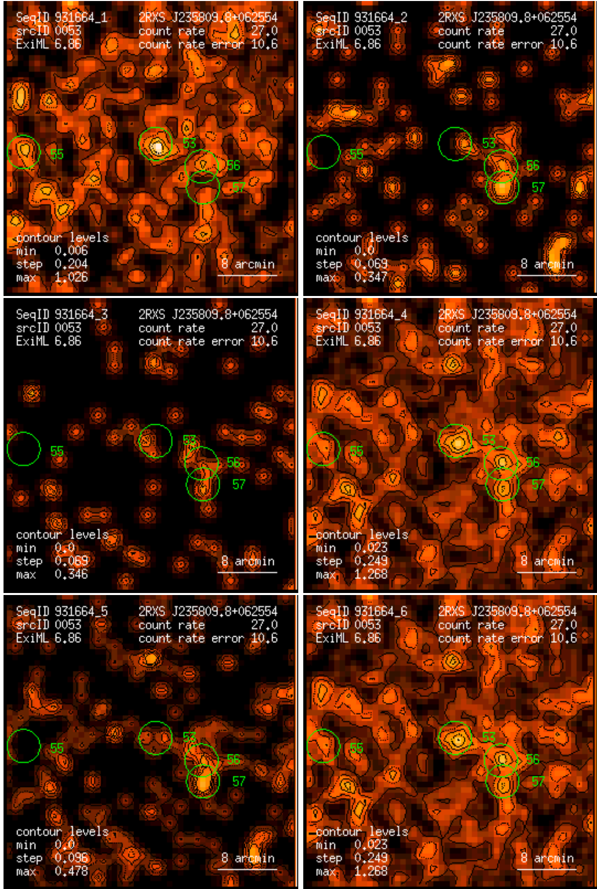
Figure 53: RASS 931664: detection 0053: band rate images, Gaussian filter: (1) PSPC channels 11 – 41, (2) 52 – 90, (3) 91 – 201, (4) 11 – 235, (5) 52 – 201, (6) 11 – 201. Broad band rates in counts/ks. Band rate contour levels in counts/ks/arcmin 2 .
