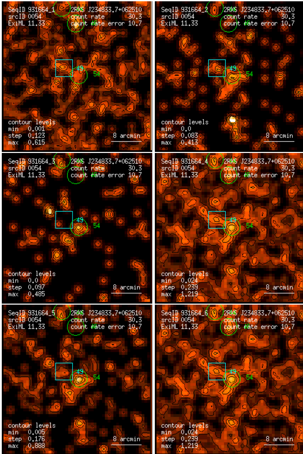
Figure 54: RASS 931664: detection 0054: band rate images, Gaussian filter: (1) PSPC channels 11 – 41, (2) 52 – 90, (3) 91 – 201, (4) 11 – 235, (5) 52 – 201, (6) 11 – 201. Broad band rates in counts/ks. Band rate contour levels in counts/ks/arcmin 2 .
