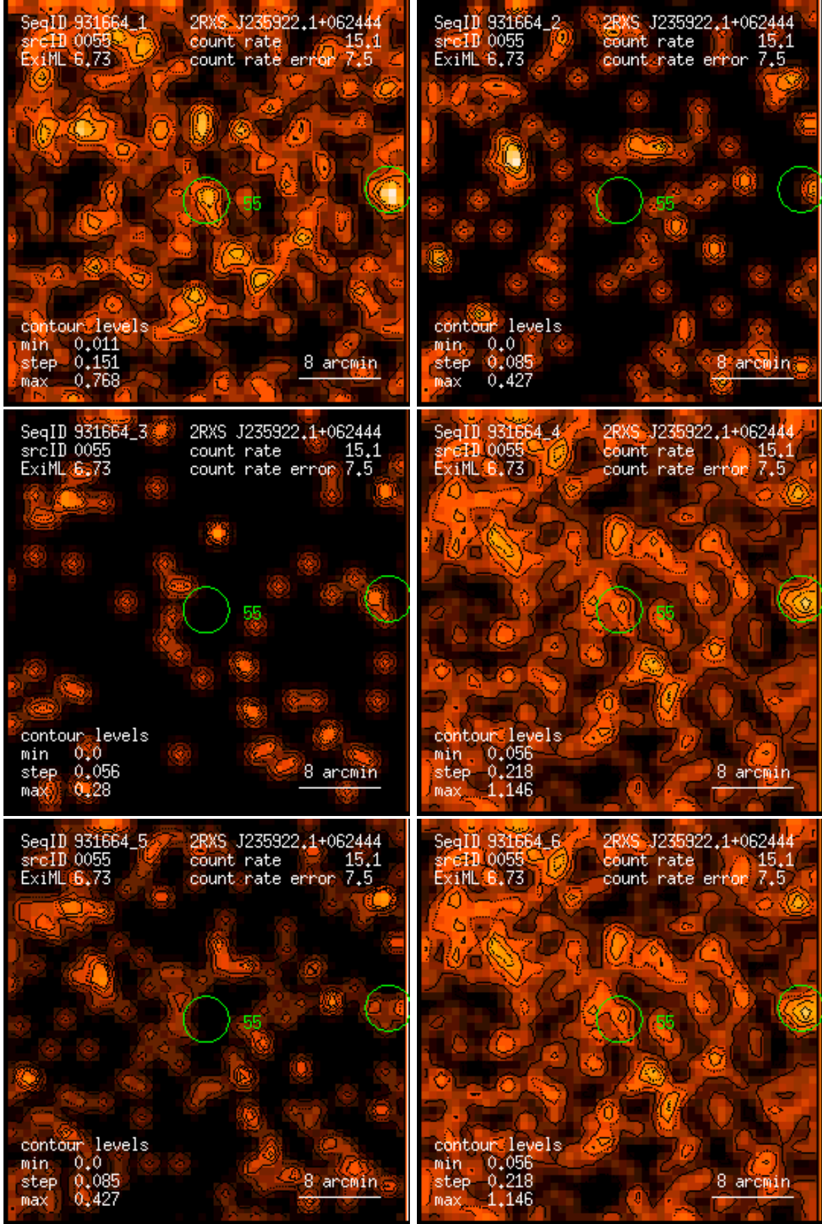
Figure 55: RASS 931664: detection 0055: band rate images, Gaussian filter: (1) PSPC channels 11 – 41, (2) 52 – 90, (3) 91 – 201, (4) 11 – 235, (5) 52 – 201, (6) 11 – 201. Broad band rates in counts/ks. Band rate contour levels in counts/ks/arcmin 2 .
