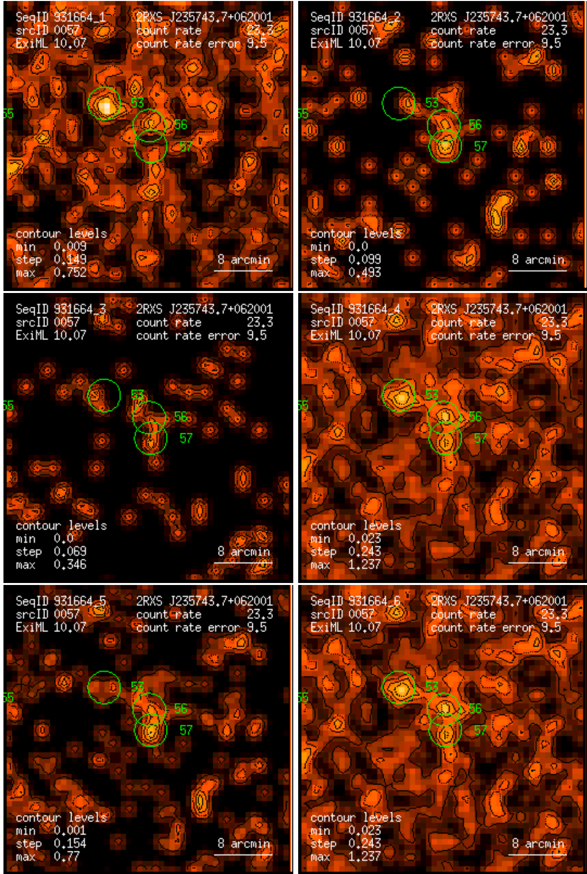
Figure 57: RASS 931664: detection 0057: band rate images, Gaussian filter: (1) PSPC channels 11 – 41, (2) 52 – 90, (3) 91 – 201, (4) 11 – 235, (5) 52 – 201, (6) 11 – 201. Broad band rates in counts/ks. Band rate contour levels in counts/ks/arcmin 2 .
