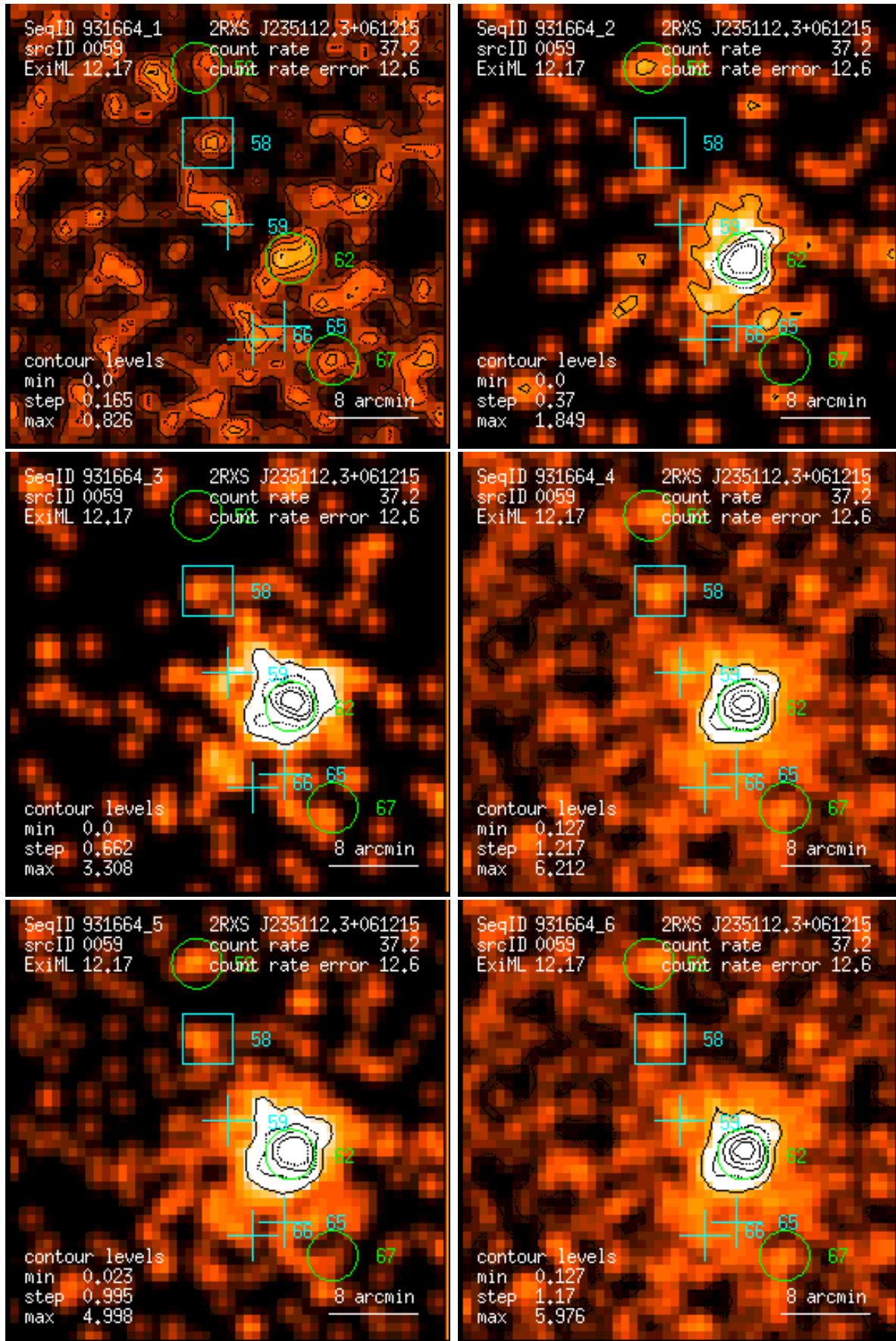
Figure 59: RASS 931664: detection 0059: band rate images, Gaussian filter: (1) PSPC channels 11 – 41, (2) 52 – 90, (3) 91 – 201, (4) 11 – 235, (5) 52 – 201, (6) 11 – 201. Broad band rates in counts/ks. Band rate contour levels in counts/ks/arcmin 2 .
