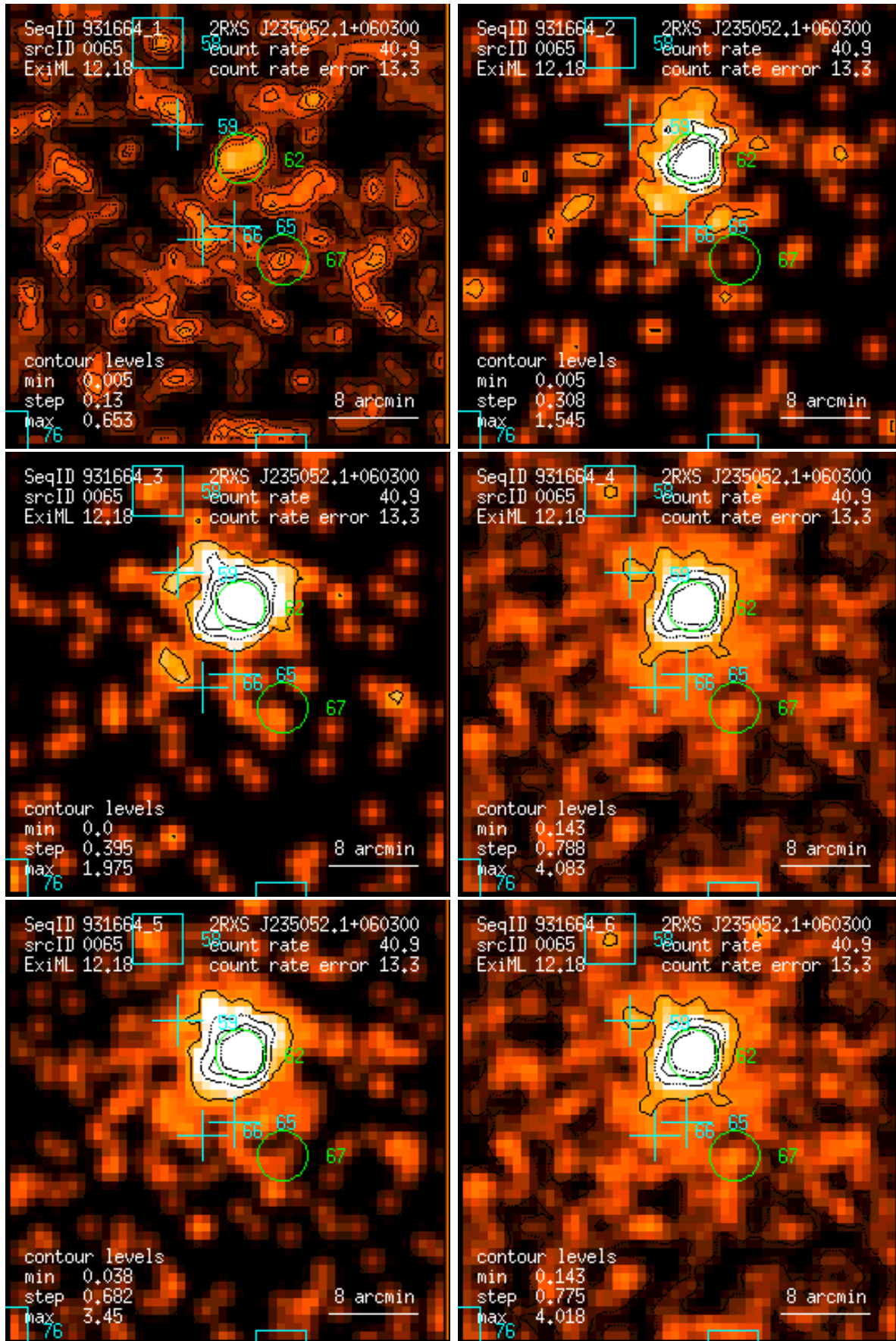
Figure 65: RASS 931664: detection 0065: band rate images, Gaussian filter: (1) PSPC channels 11 – 41, (2) 52 – 90, (3) 91 – 201, (4) 11 – 235, (5) 52 – 201, (6) 11 – 201. Broad band rates in counts/ks. Band rate contour levels in counts/ks/arcmin 2 .
