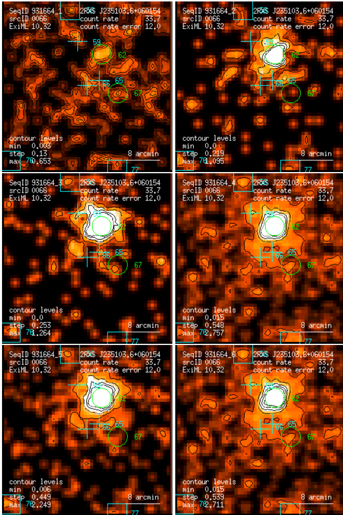
Figure 66: RASS 931664: detection 0066: band rate images, Gaussian filter: (1) PSPC channels 11 – 41, (2) 52 – 90, (3) 91 – 201, (4) 11 – 235, (5) 52 – 201, (6) 11 – 201. Broad band rates in counts/ks. Band rate contour levels in counts/ks/arcmin 2 .
