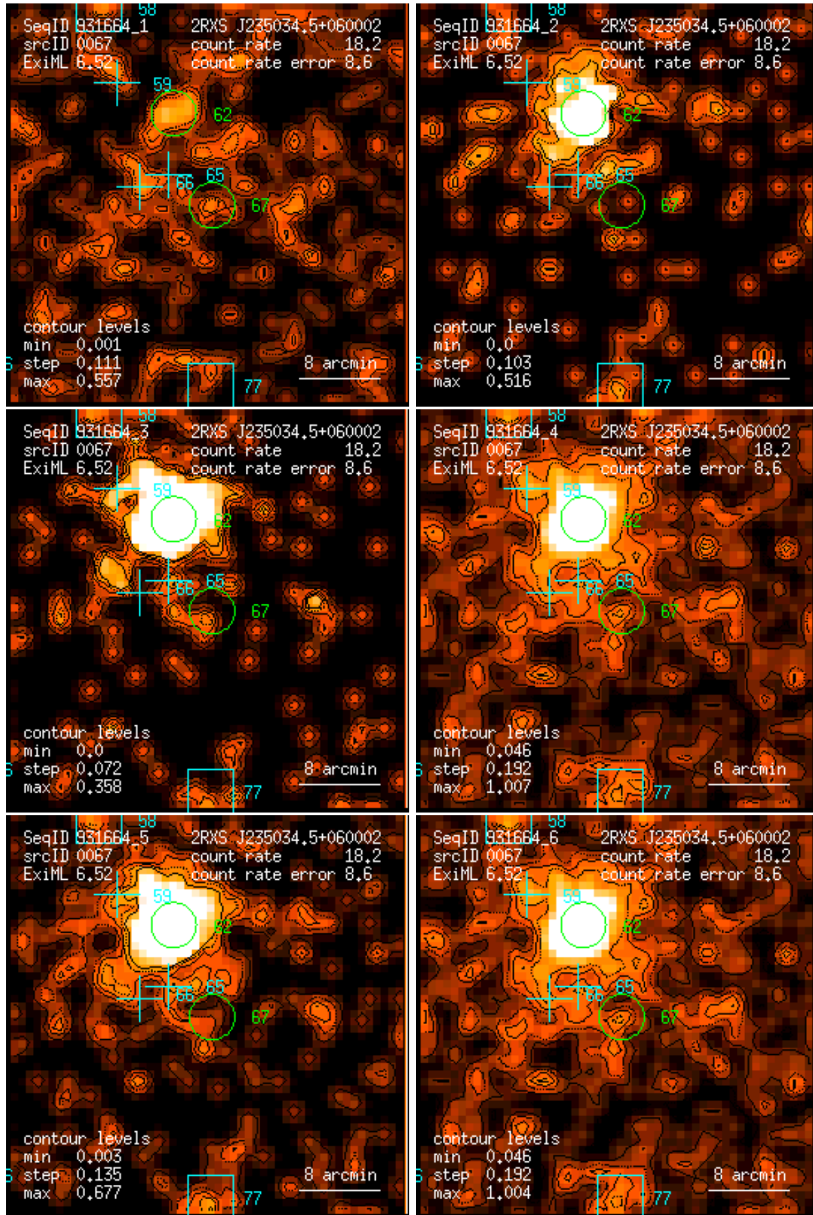
Figure 67: RASS 931664: detection 0067: band rate images, Gaussian filter: (1) PSPC channels 11 – 41, (2) 52 – 90, (3) 91 – 201, (4) 11 – 235, (5) 52 – 201, (6) 11 – 201. Broad band rates in counts/ks. Band rate contour levels in counts/ks/arcmin 2 .
