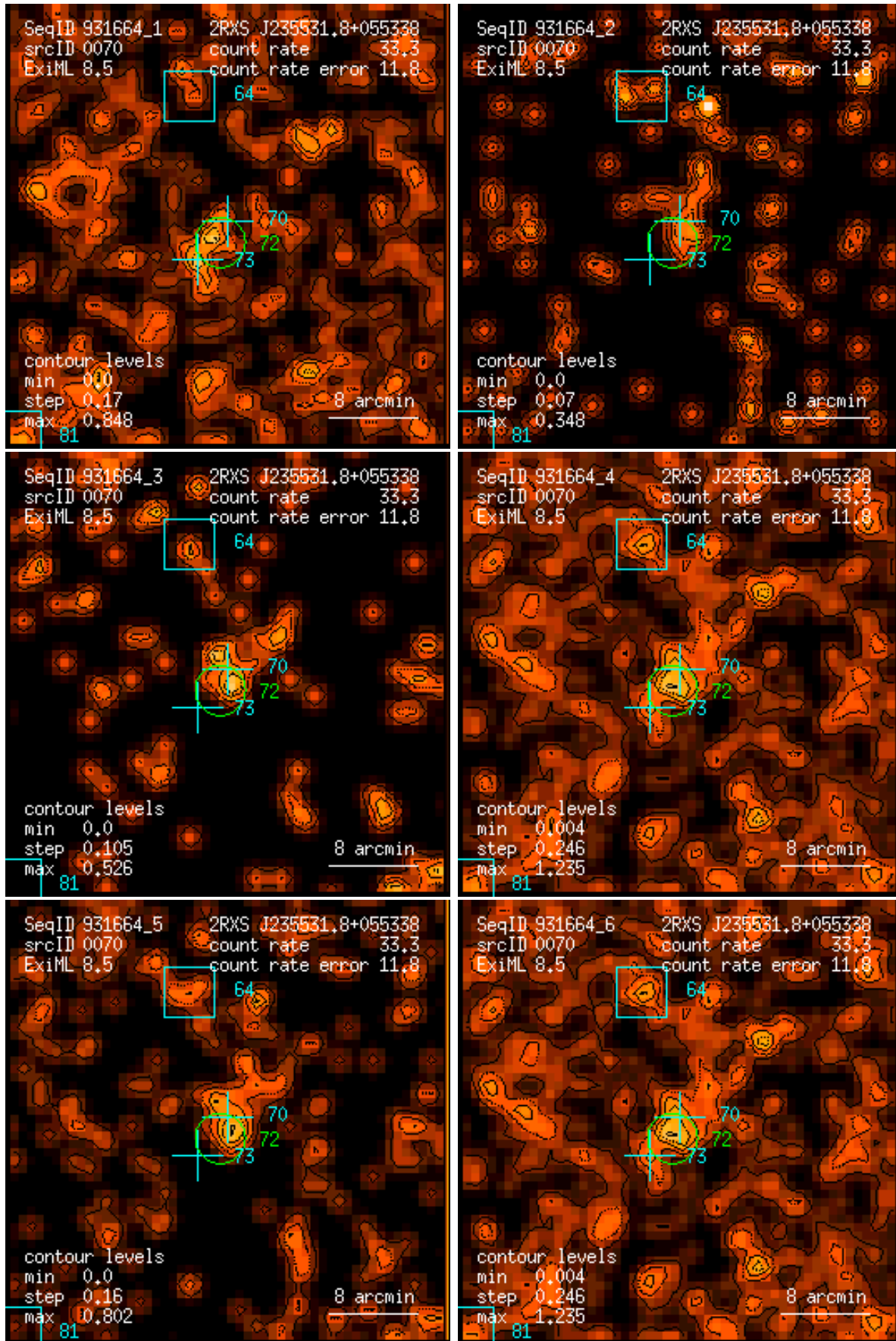
Figure 70: RASS 931664: detection 0070: band rate images, Gaussian filter: (1) PSPC channels 11 – 41, (2) 52 – 90, (3) 91 – 201, (4) 11 – 235, (5) 52 – 201, (6) 11 – 201. Broad band rates in counts/ks. Band rate contour levels in counts/ks/arcmin 2 .
