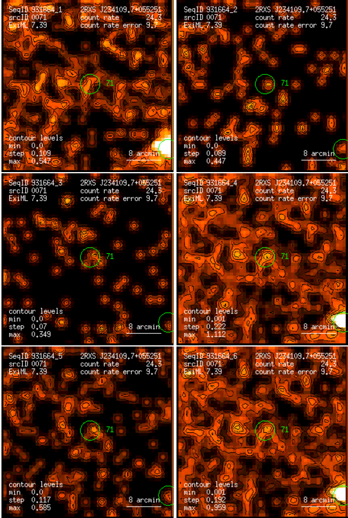
Figure 71: RASS 931664: detection 0071: band rate images, Gaussian filter: (1) PSPC channels 11 – 41, (2) 52 – 90, (3) 91 – 201, (4) 11 – 235, (5) 52 – 201, (6) 11 – 201. Broad band rates in counts/ks. Band rate contour levels in counts/ks/arcmin 2 .
