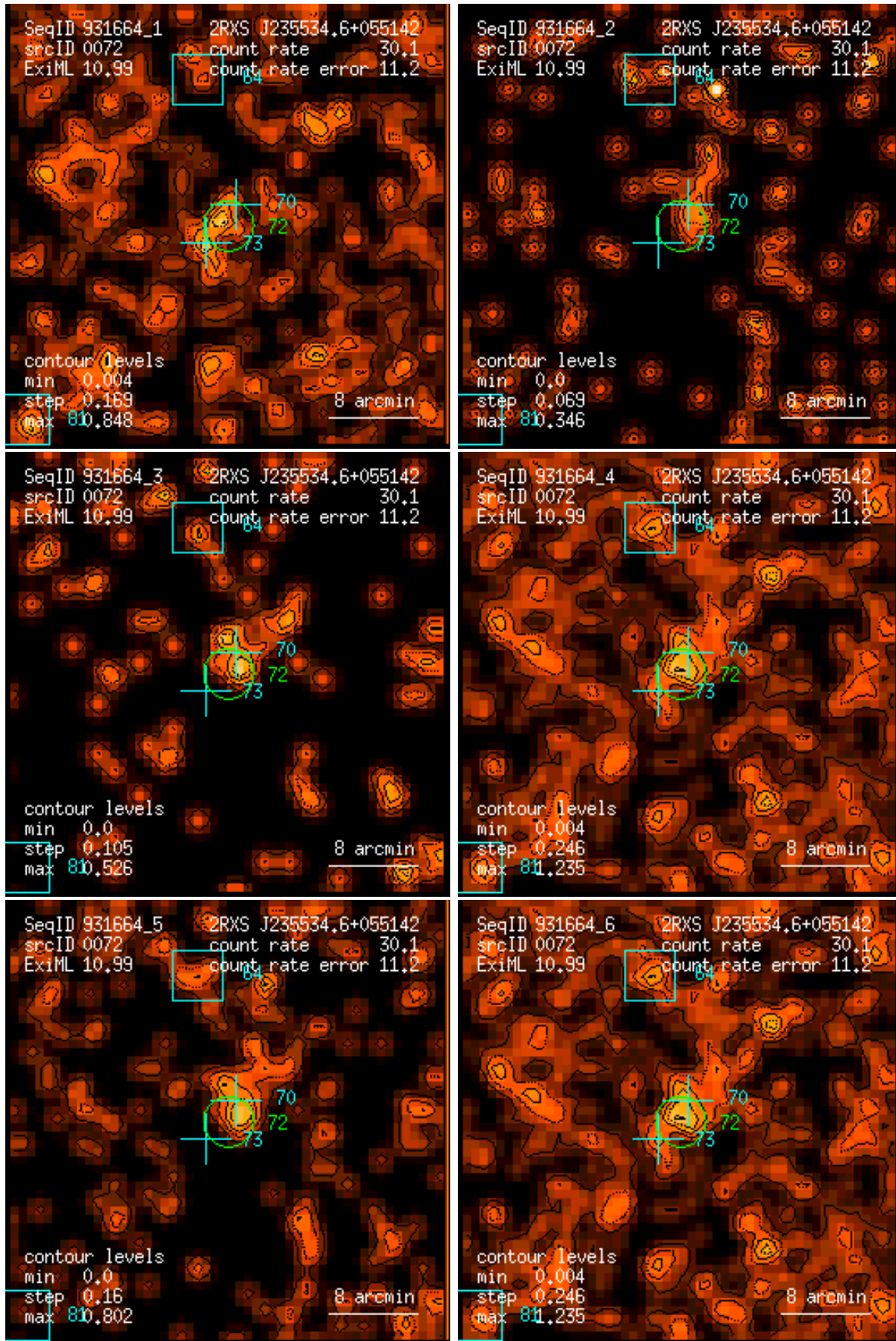
Figure 72: RASS 931664: detection 0072: band rate images, Gaussian filter: (1) PSPC channels 11 – 41, (2) 52 – 90, (3) 91 – 201, (4) 11 – 235, (5) 52 – 201, (6) 11 – 201. Broad band rates in counts/ks. Band rate contour levels in counts/ks/arcmin 2 .
