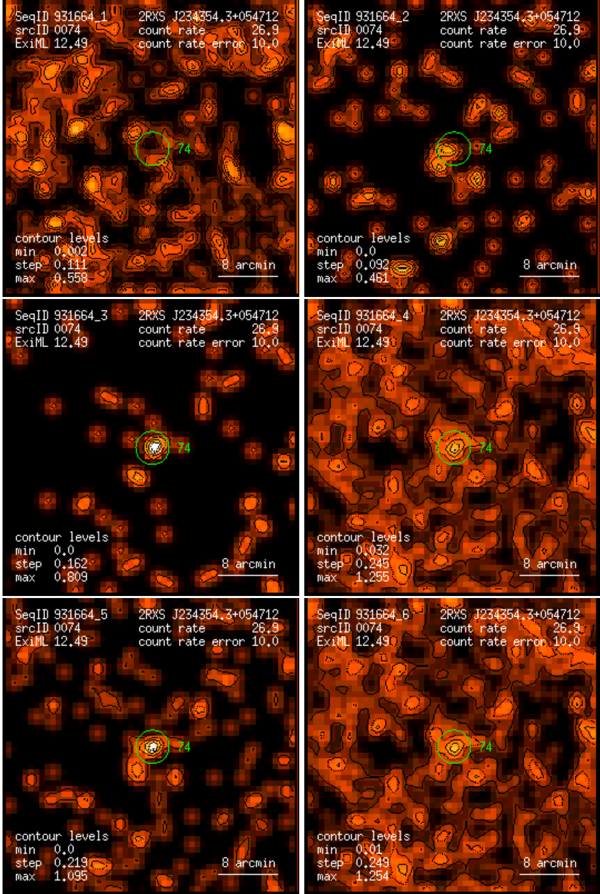
Figure 74: RASS 931664: detection 0074: band rate images, Gaussian filter: (1) PSPC channels 11 – 41, (2) 52 – 90, (3) 91 – 201, (4) 11 – 235, (5) 52 – 201, (6) 11 – 201. Broad band rates in counts/ks. Band rate contour levels in counts/ks/arcmin 2 .
