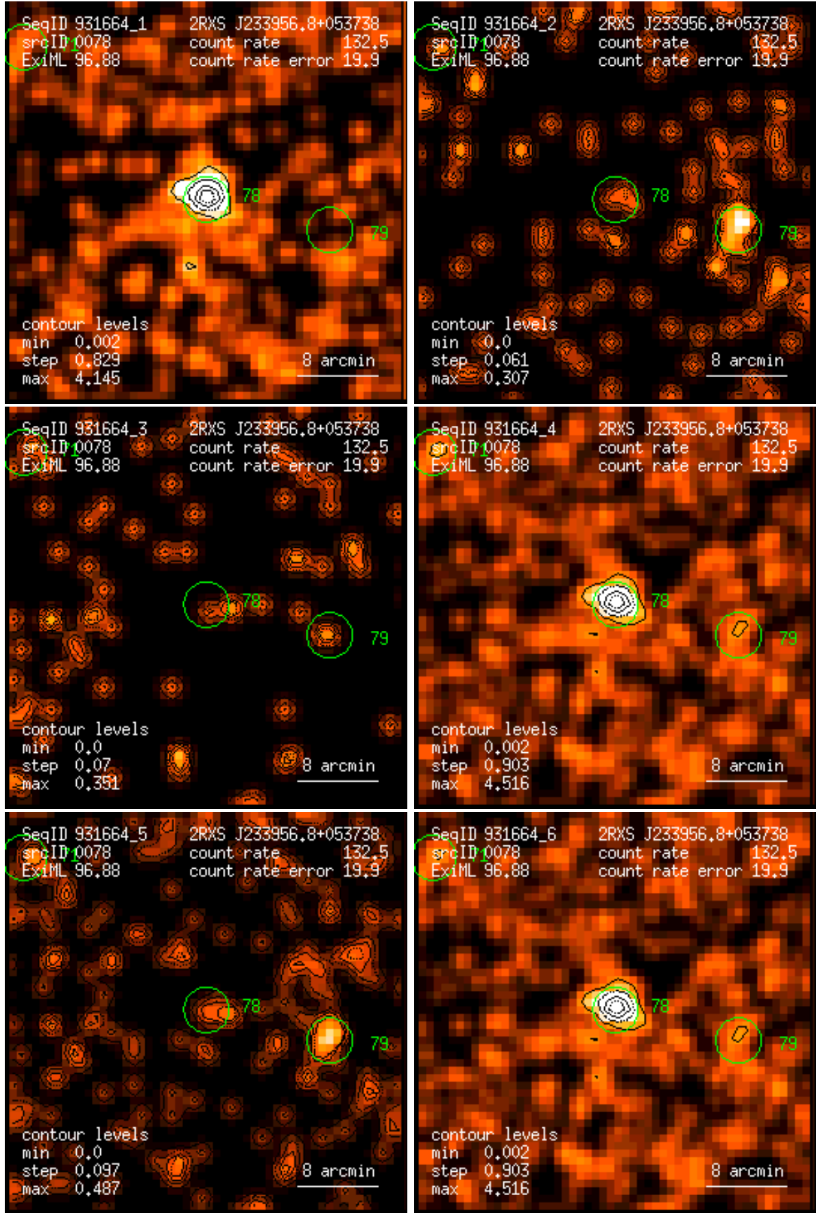
Figure 78: RASS 931664: detection 0078: band rate images, Gaussian filter: (1) PSPC channels 11 – 41, (2) 52 – 90, (3) 91 – 201, (4) 11 – 235, (5) 52 – 201, (6) 11 – 201. Broad band rates in counts/ks. Band rate contour levels in counts/ks/arcmin 2 .
