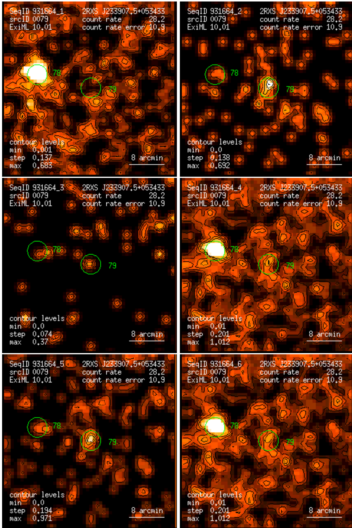
Figure 79: RASS 931664: detection 0079: band rate images, Gaussian filter: (1) PSPC channels 11 – 41, (2) 52 – 90, (3) 91 – 201, (4) 11 – 235, (5) 52 – 201, (6) 11 – 201. Broad band rates in counts/ks. Band rate contour levels in counts/ks/arcmin 2 .
