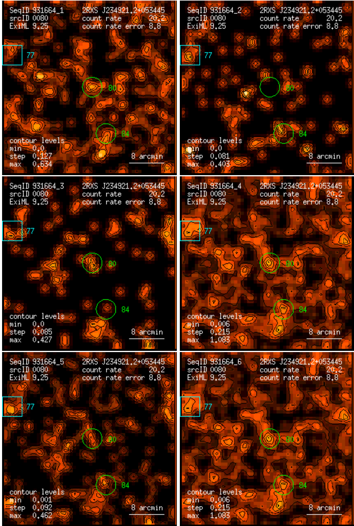
Figure 80: RASS 931664: detection 0080: band rate images, Gaussian filter: (1) PSPC channels 11 – 41, (2) 52 – 90, (3) 91 – 201, (4) 11 – 235, (5) 52 – 201, (6) 11 – 201. Broad band rates in counts/ks. Band rate contour levels in counts/ks/arcmin 2 .
