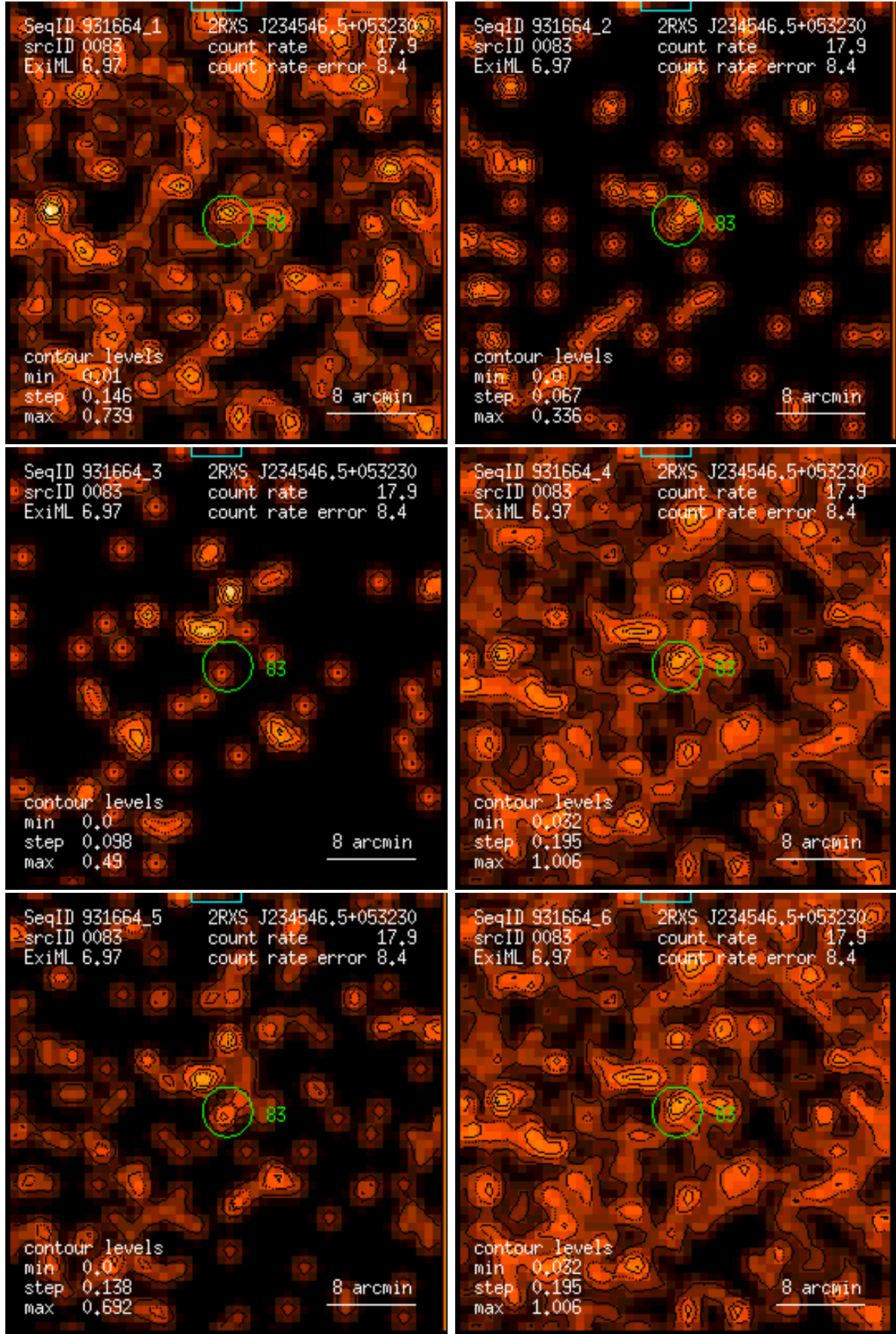
Figure 83: RASS 931664: detection 0083: band rate images, Gaussian filter: (1) PSPC channels 11 – 41, (2) 52 – 90, (3) 91 – 201, (4) 11 – 235, (5) 52 – 201, (6) 11 – 201. Broad band rates in counts/ks. Band rate contour levels in counts/ks/arcmin 2 .
