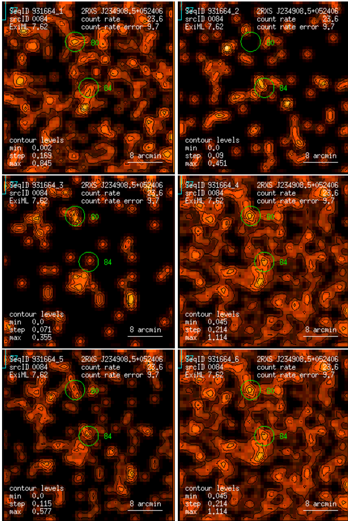
Figure 84: RASS 931664: detection 0084: band rate images, Gaussian filter: (1) PSPC channels 11 – 41, (2) 52 – 90, (3) 91 – 201, (4) 11 – 235, (5) 52 – 201, (6) 11 – 201. Broad band rates in counts/ks. Band rate contour levels in counts/ks/arcmin 2 .
