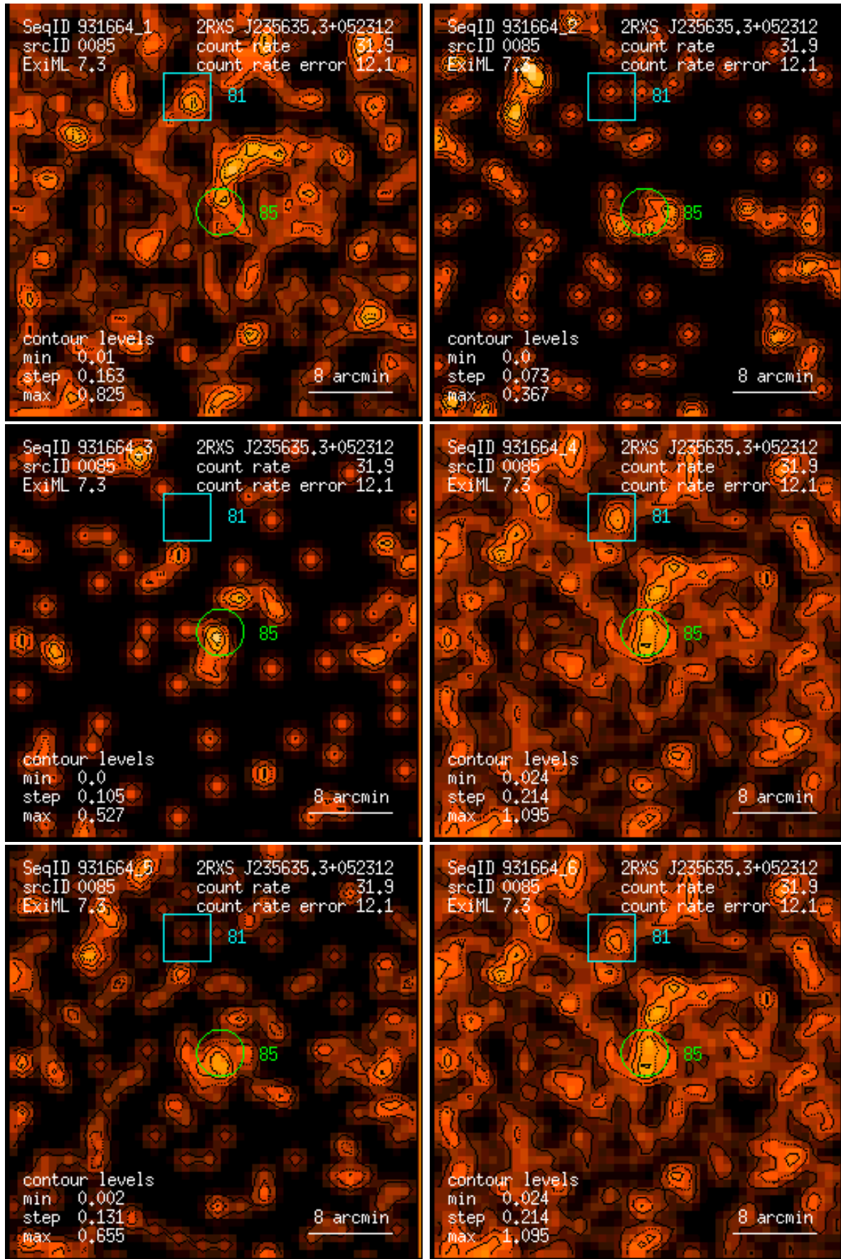
Figure 85: RASS 931664: detection 0085: band rate images, Gaussian filter: (1) PSPC channels 11 – 41, (2) 52 – 90, (3) 91 – 201, (4) 11 – 235, (5) 52 – 201, (6) 11 – 201. Broad band rates in counts/ks. Band rate contour levels in counts/ks/arcmin 2 .
